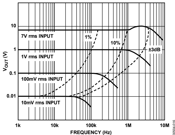
Figure 18. High Frequency Response
