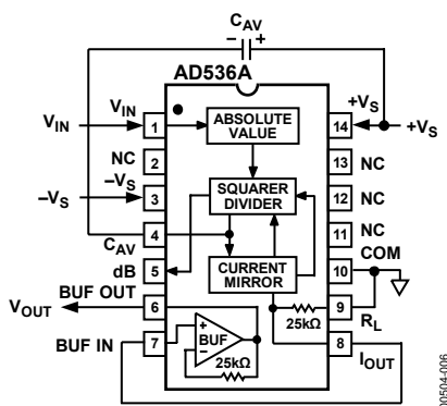
Figure 6. TO-116 and Q-14 Standard RMS Connection
