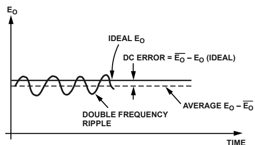
Figure 11. Typical Output Waveform for Sinusoidal Input
