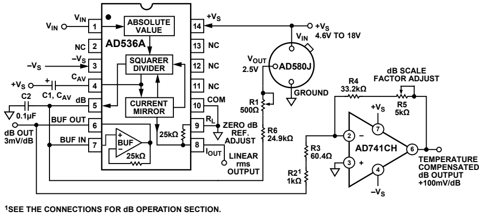
Figure 17. dB Connection
