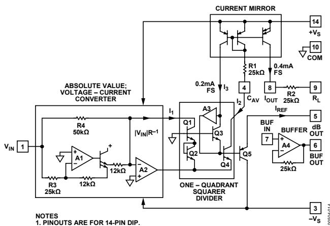
Figure 16. Simplified Schematic
