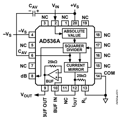
Figure 8. LCC Standard RMS Connection
