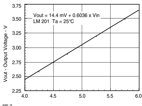
Figure 19. Transfer Gain
