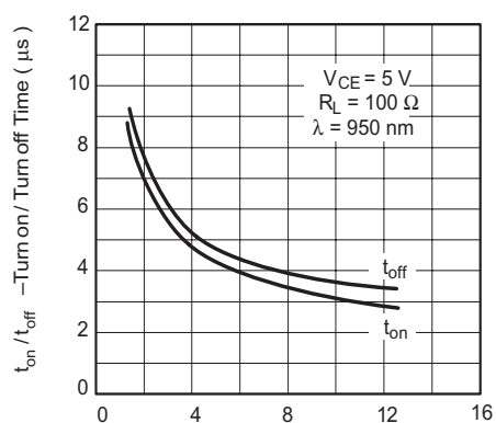
94 8238 I_C - Collector Current (mA)
