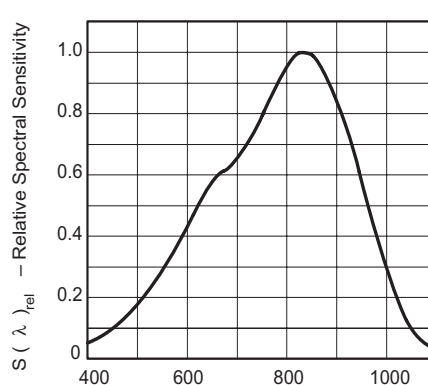
94 8241 \lambda - Wavelength (nm)
