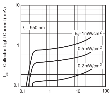
94 8242 V_{CE} - Collector Emitter Voltage (V)
