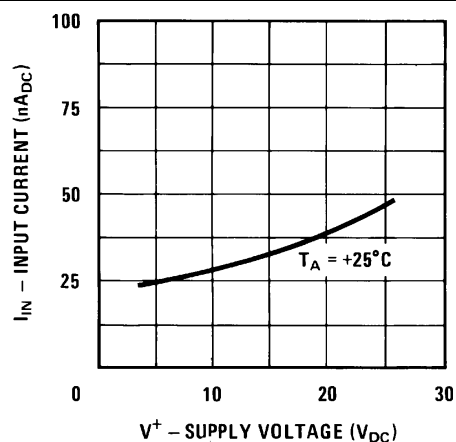
Figure 13. Input Current (LM2902 Only)
