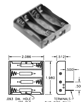
Holds Four (4) "AAA" Cells in Series
