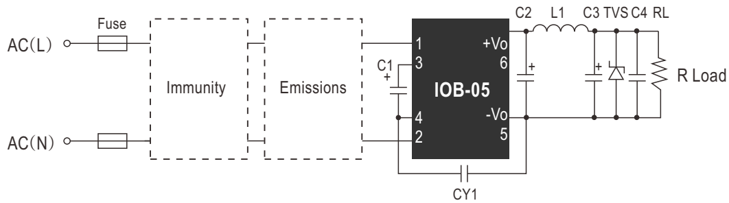
IOB-05 Series additional component selection guide (no EMC devices)
