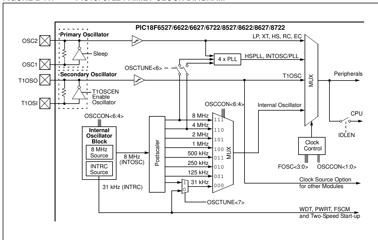
FIGURE 2-11: PIC18F8722 FAMILY CLOCK DIAGRAM
