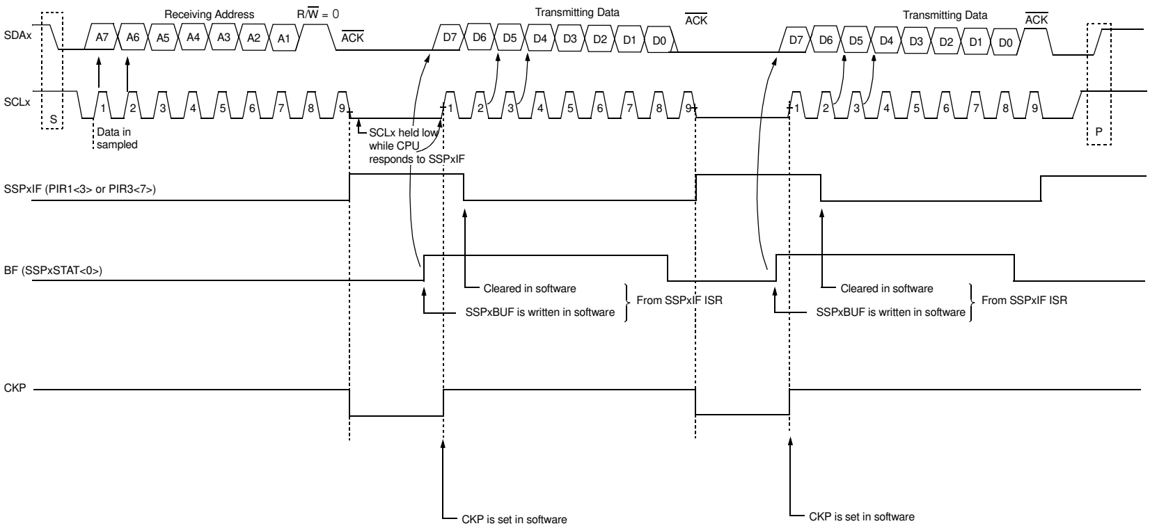
FIGURE 19-9: I 2 C™ SLAVE MODE TIMING (TRANSMISSION, 7-BIT ADDRESS)
