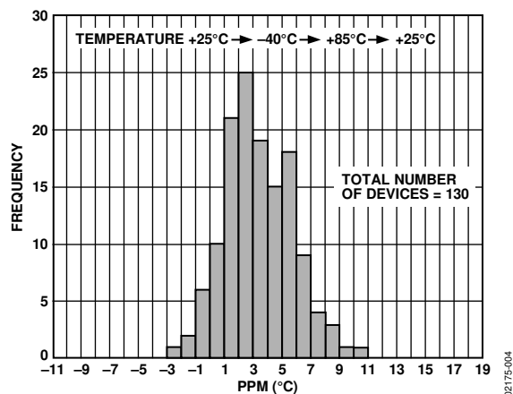
Figure 4. ADR380 Output Voltage Temperature Coefficient
