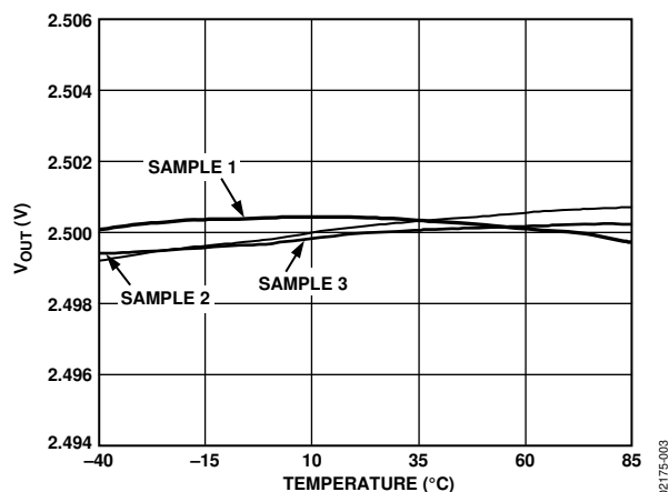
Figure 3. ADR381 Output Voltage vs. Temperature
