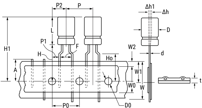
Fig. 2 (Diameter for \Phi 5 to \Phi 8 ) 5 – 8 mm formed to 5 mm DA
