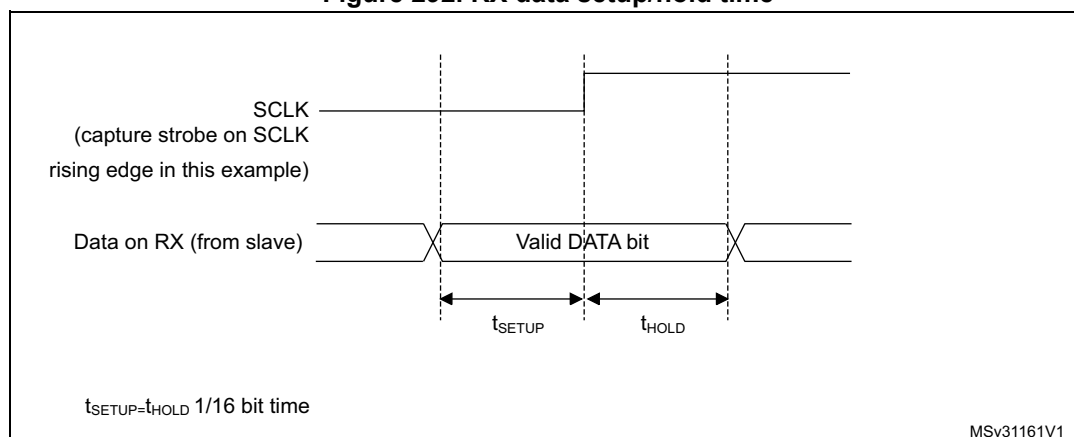
Figure 292. RX data setup/hold time
