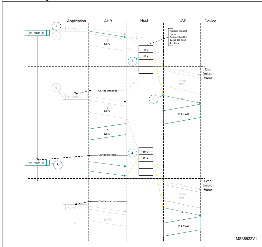
Figure 424. Normal isochronous IN transactions - DMA mode
