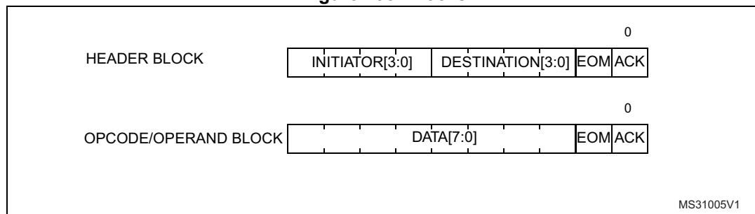
Figure 435. Blocks
