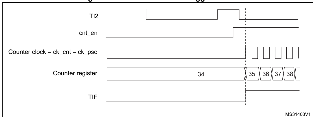
Figure 226. Control circuit in trigger mode
