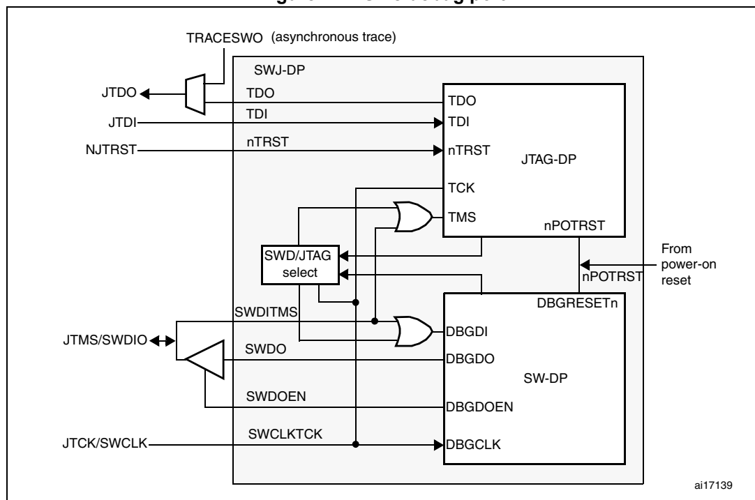
Figure 444. SWJ debug port
