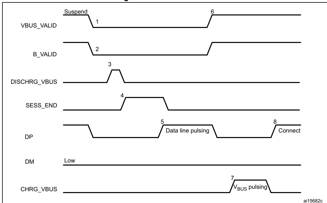
Figure 430. B-device SRP
