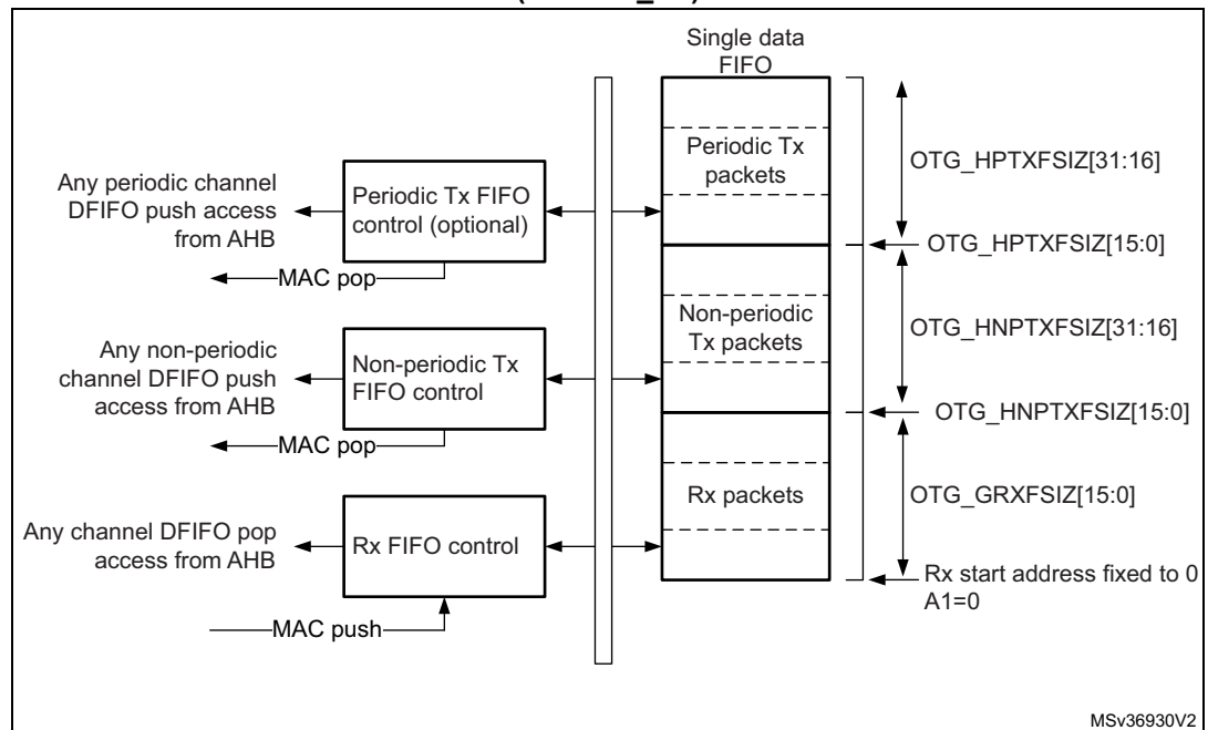
Figure 408. Host-mode FIFO address mapping and AHB FIFO access mapping (for OTG_FS)
