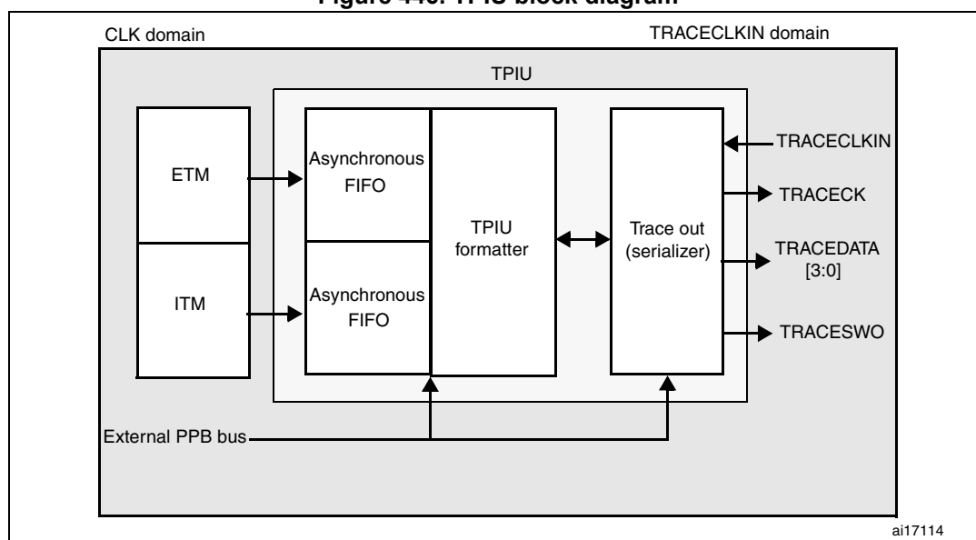
Figure 446. TPIU block diagram
