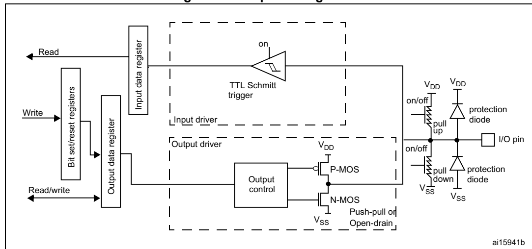
Figure 21. Output configuration
