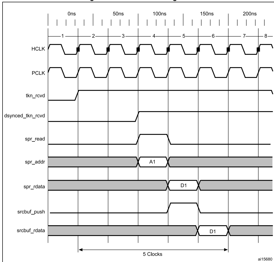
Figure 428. TRDT max timing case
