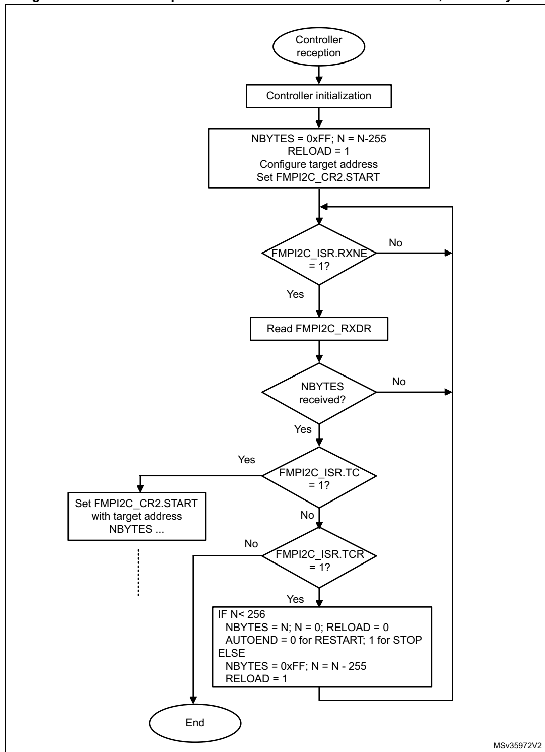
Figure 262. Transfer sequence flow for FMPI2C controller receiver, N > 255 bytes
