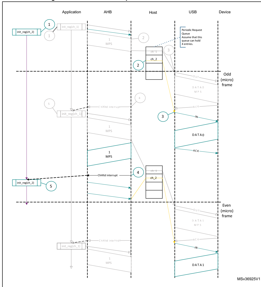
Figure 422. Normal interrupt IN transactions - DMA mode
