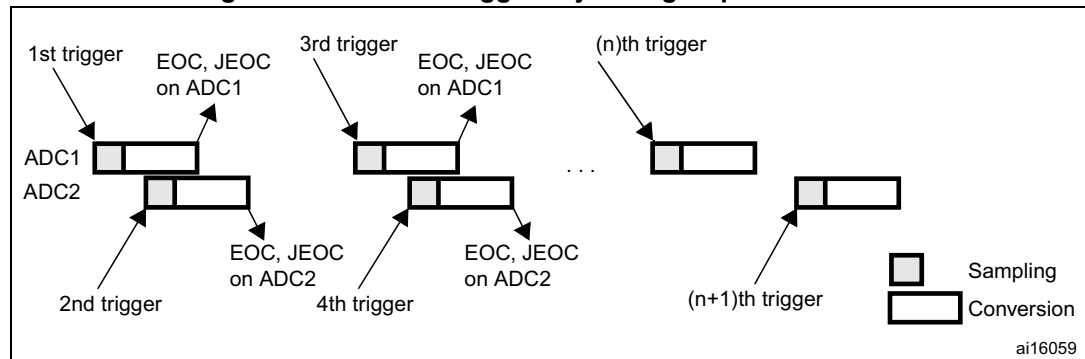
Figure 86. Alternate trigger: injected group of each ADC
