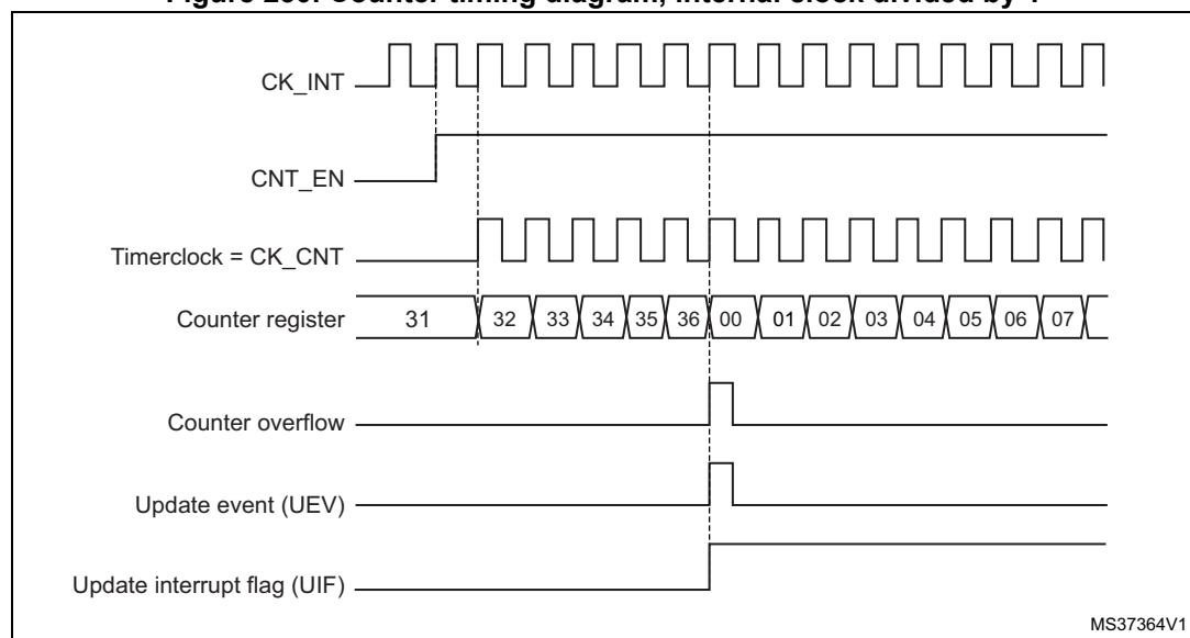
Figure 230. Counter timing diagram, internal clock divided by 1
