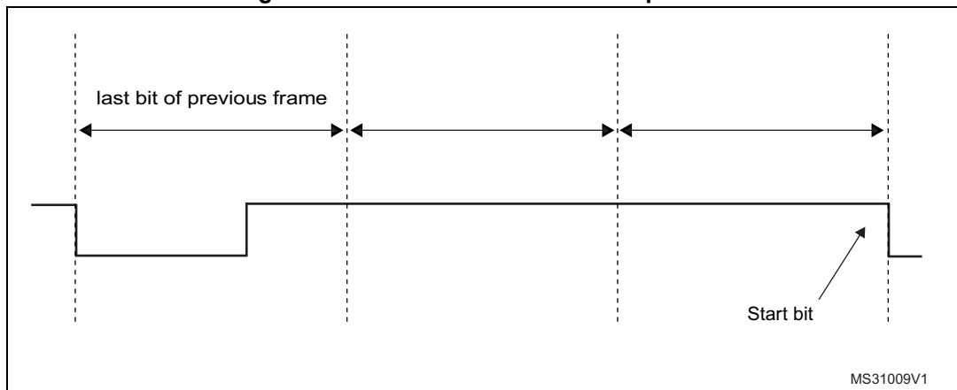
Figure 439. SFT of three nominal bit periods
