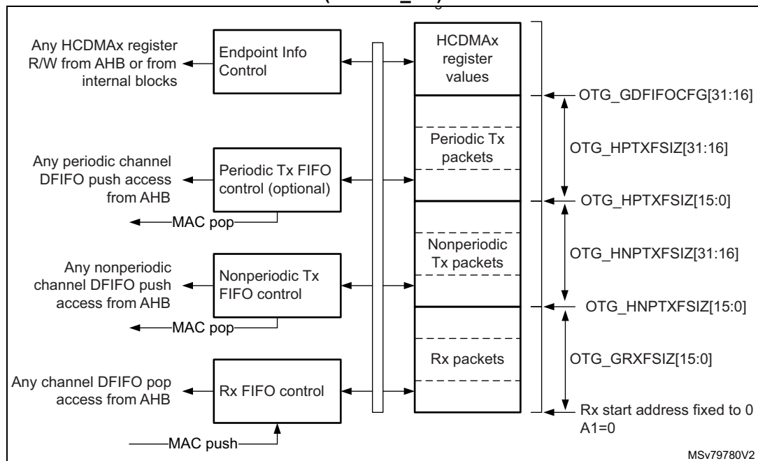
Figure 409. Host-mode FIFO address mapping and AHB FIFO access mapping (for OTG_HS)
