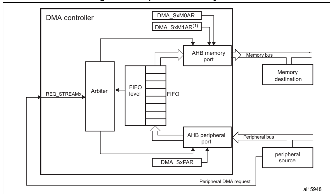
Figure 26. Peripheral-to-memory mode
