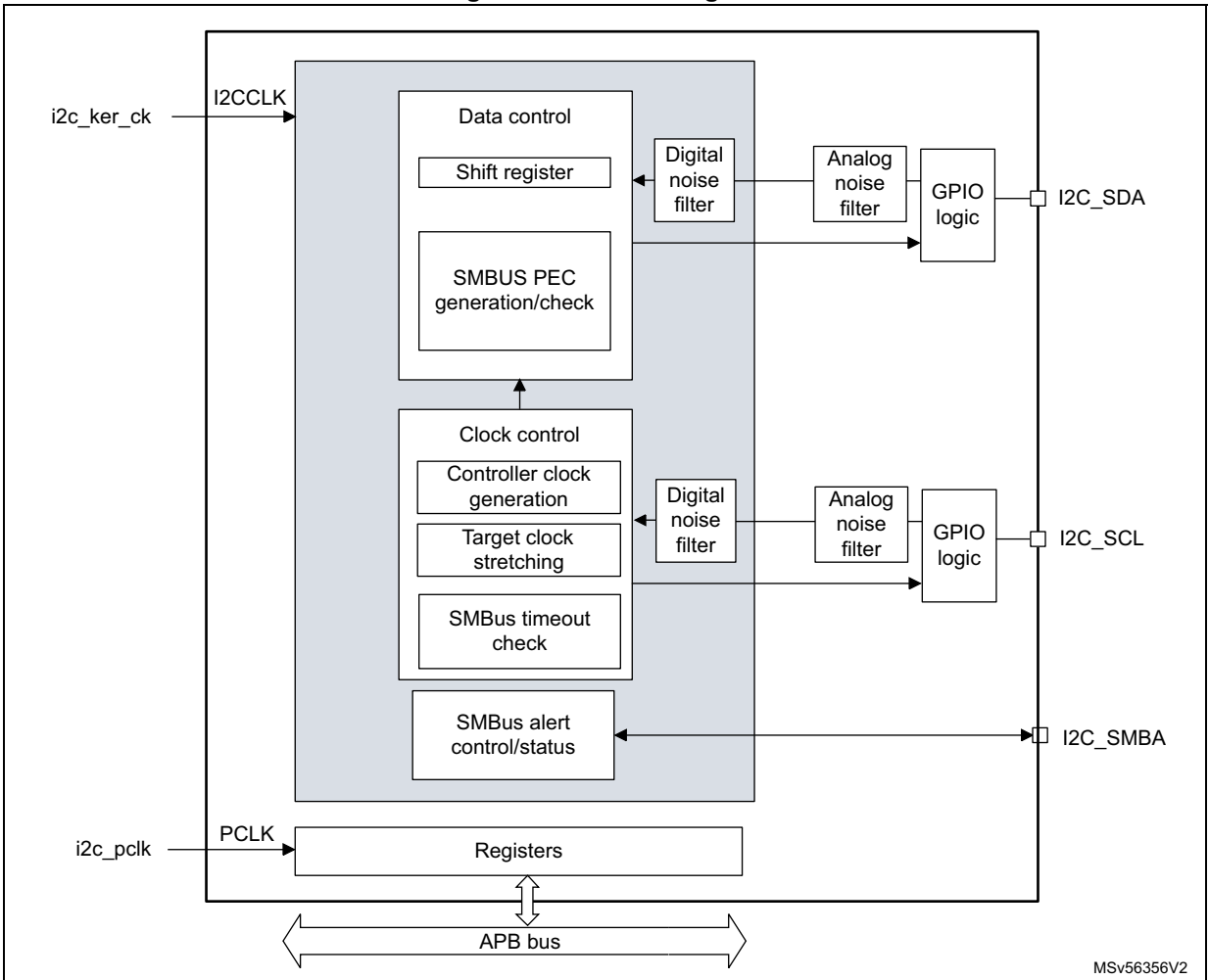
Figure 241. Block diagram
