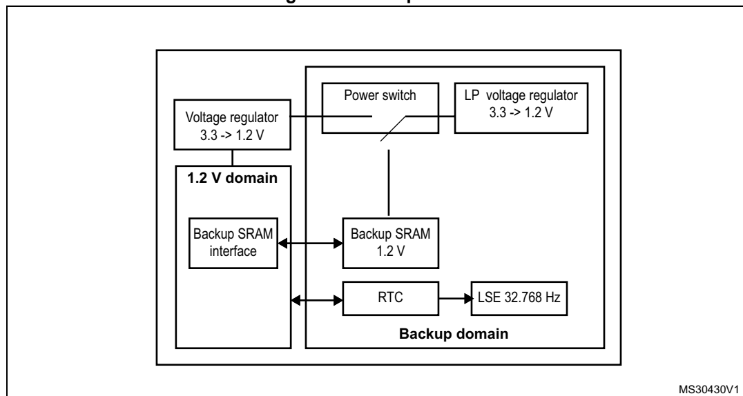
Figure 9. Backup domain
