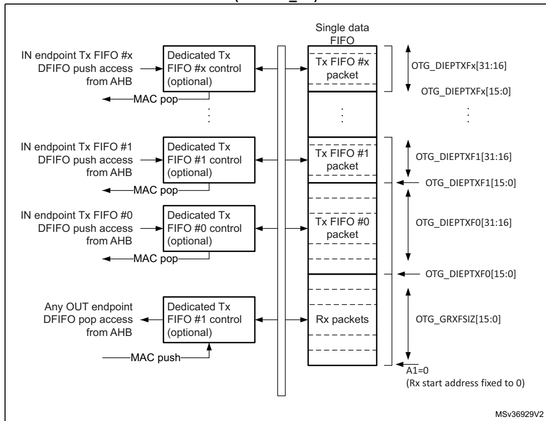
Figure 406. Device-mode FIFO address mapping and AHB FIFO access mapping (for OTG_FS)
