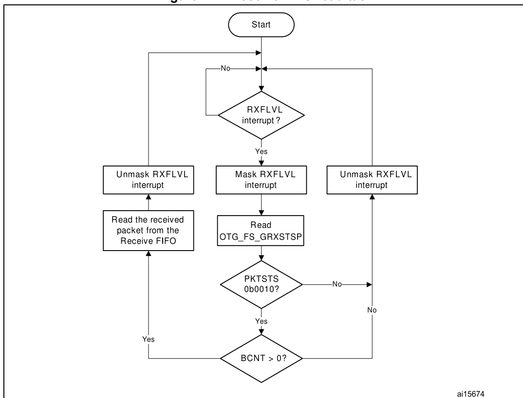
Figure 412. Receive FIFO read task
