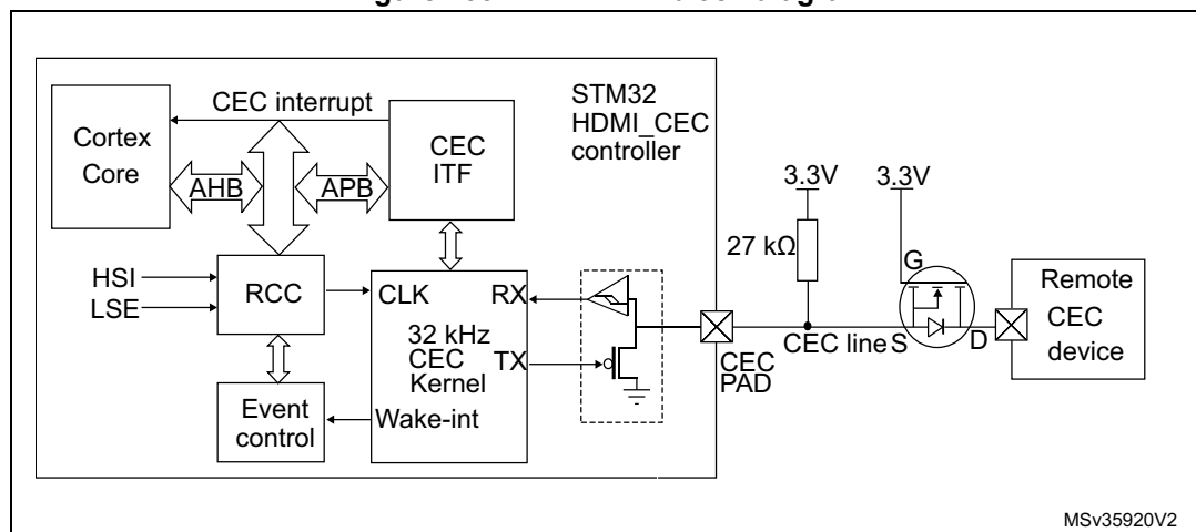
Figure 433. HDMI-CEC block diagram
