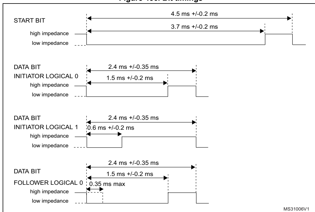
Figure 436. Bit timings
