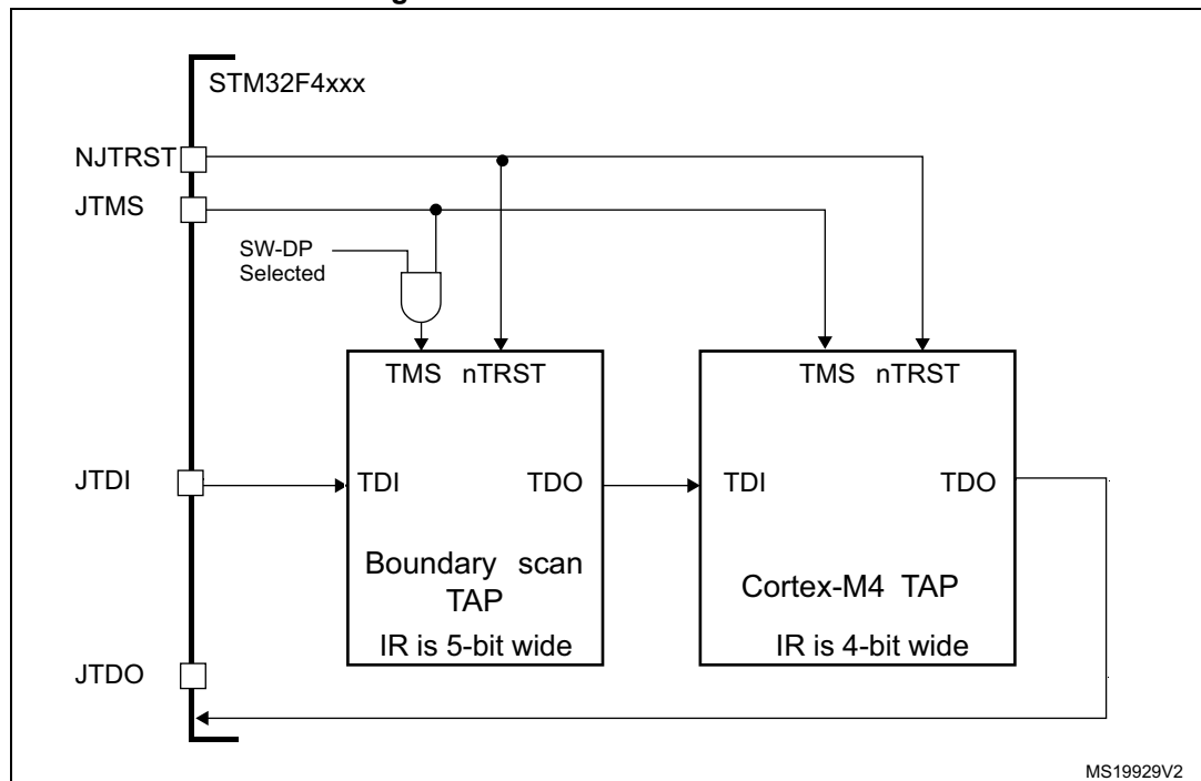
Figure 445. JTAG TAP connections
