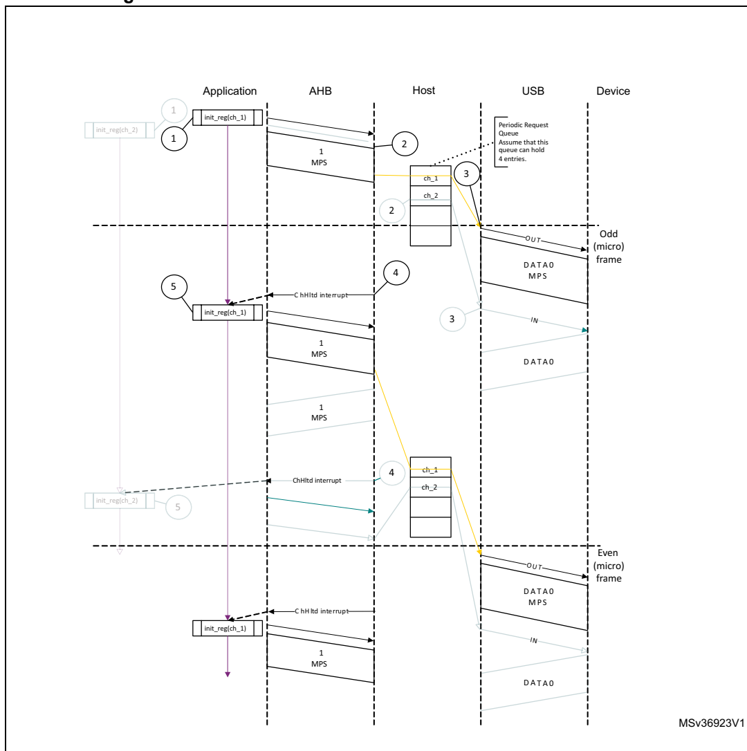
Figure 423. Normal isochronous OUT transaction - DMA mode
