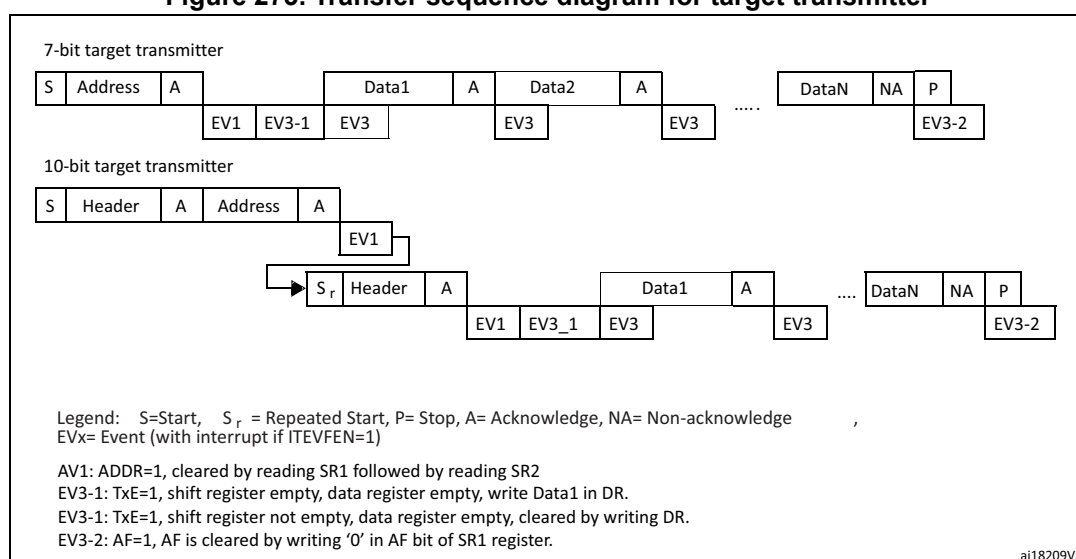
Figure 273. Transfer sequence diagram for target transmitter
