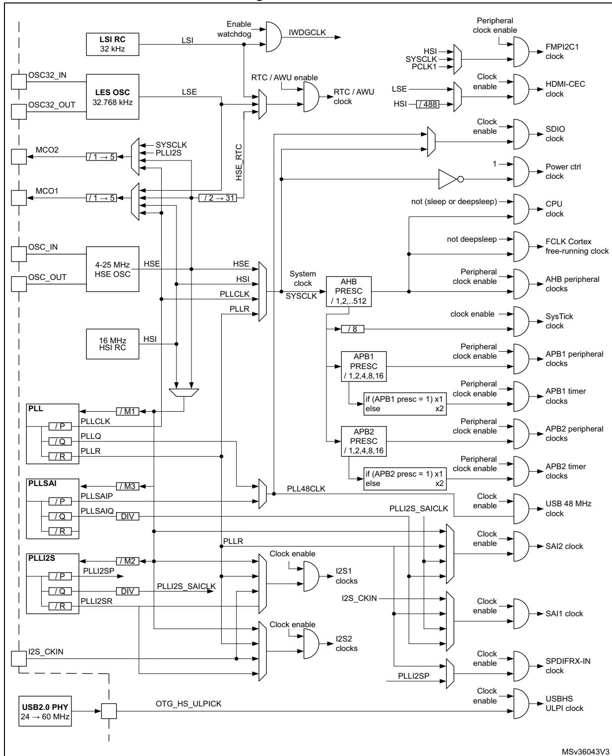
Figure 14. Clock tree
