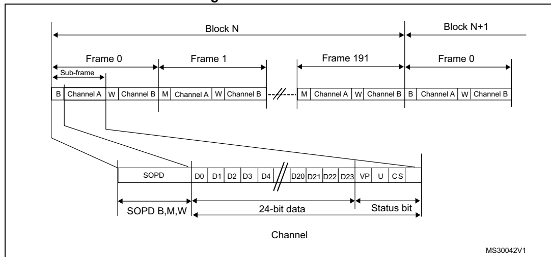
Figure 362. SPDIF format
