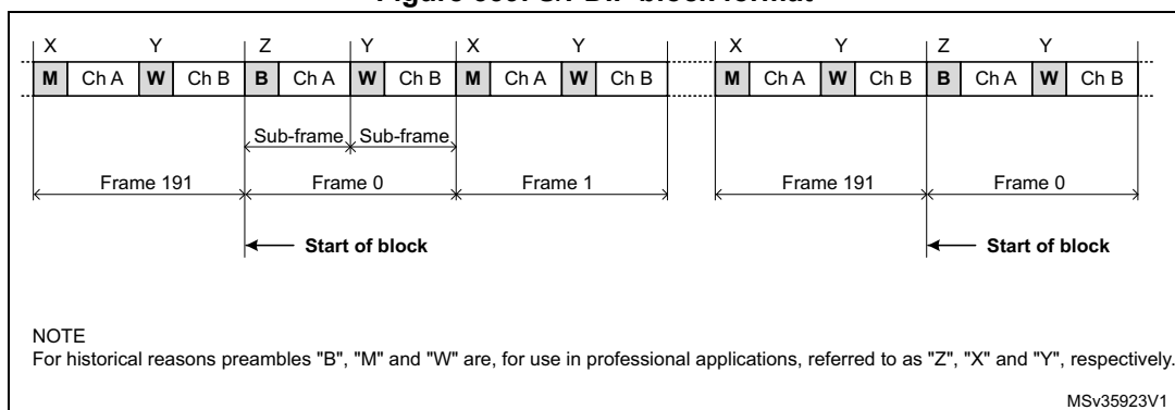
Figure 339. S/PDIF block format
