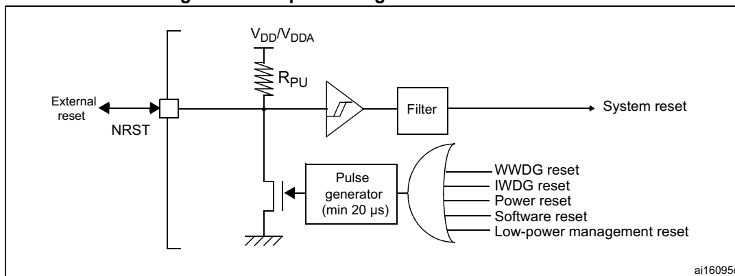
Figure 13. Simplified diagram of the reset circuit
