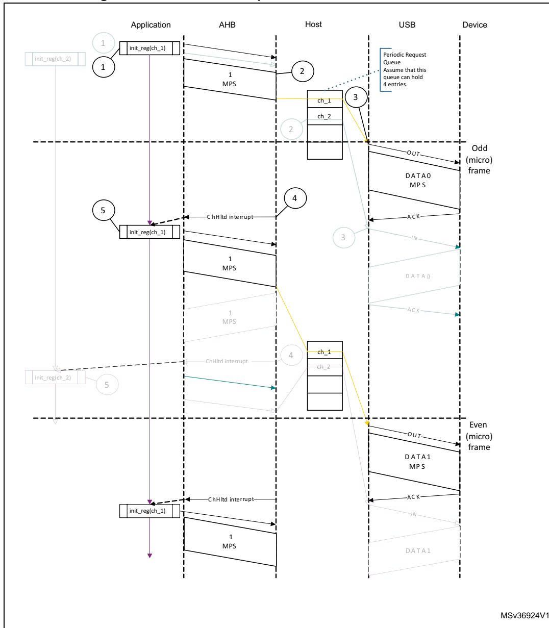
Figure 421. Normal interrupt OUT transactions - DMA mode
