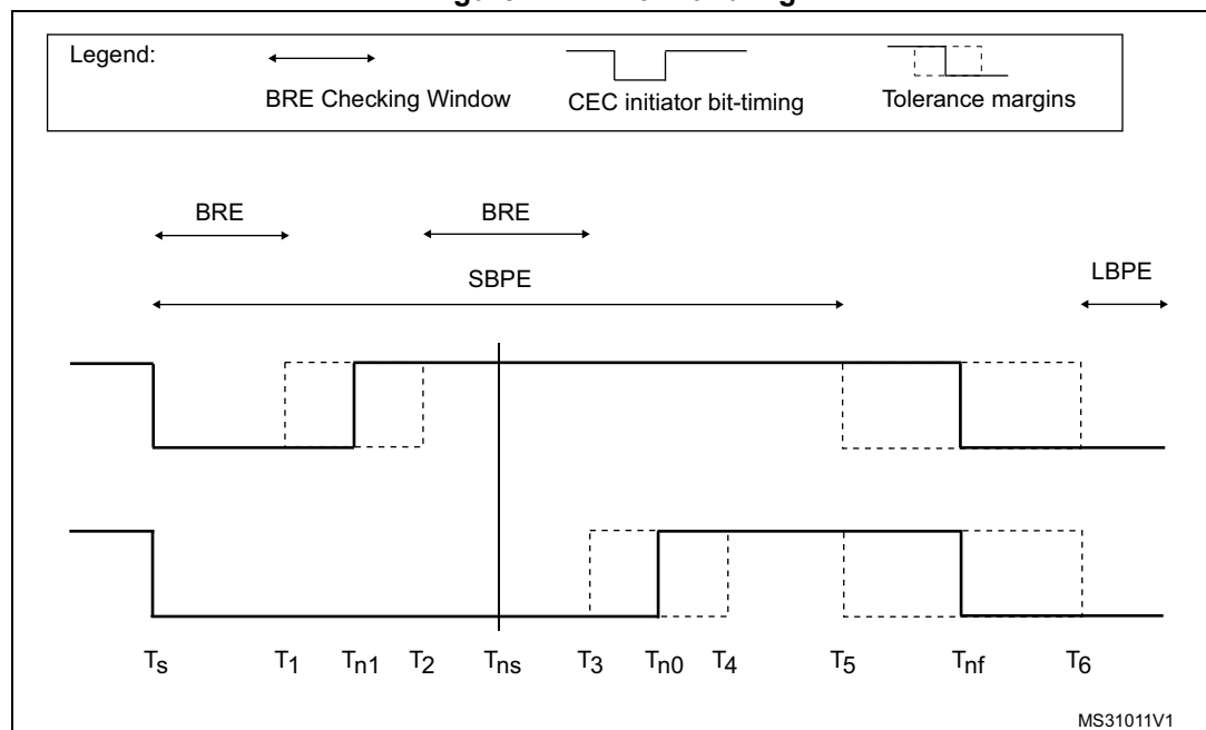
Figure 441. Error handling
