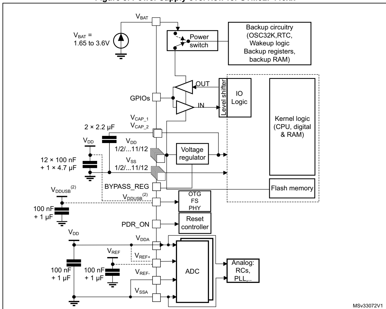
Figure 8. Power supply overview for STM32F446xx
