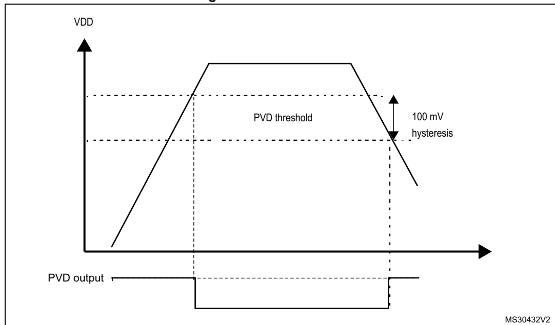
Figure 12. PVD thresholds
