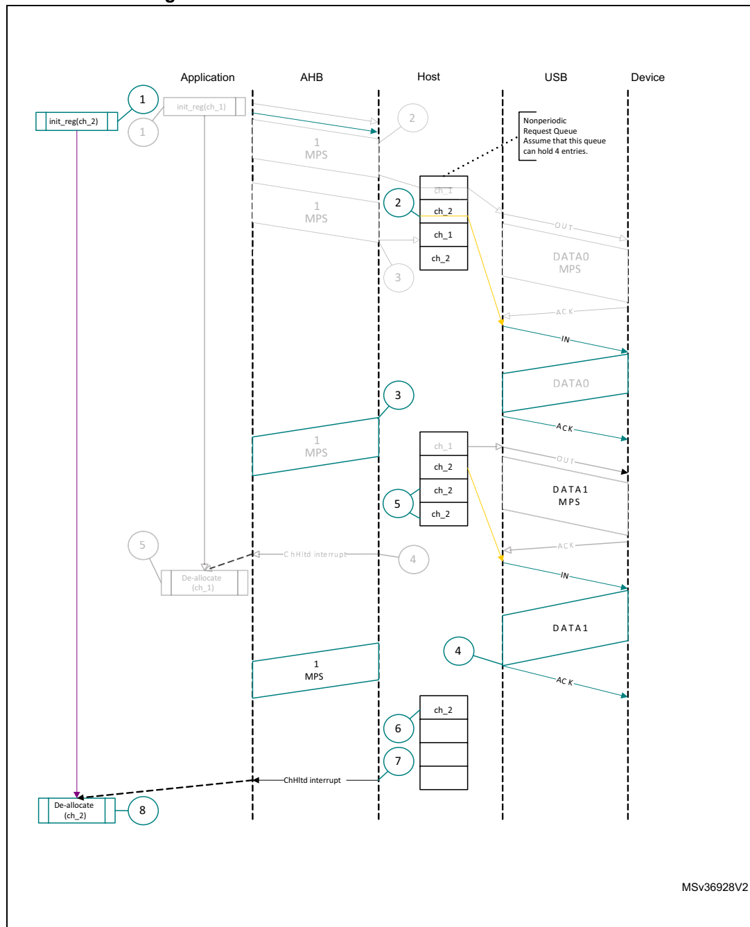
Figure 420. Normal bulk/control IN transaction - DMA
