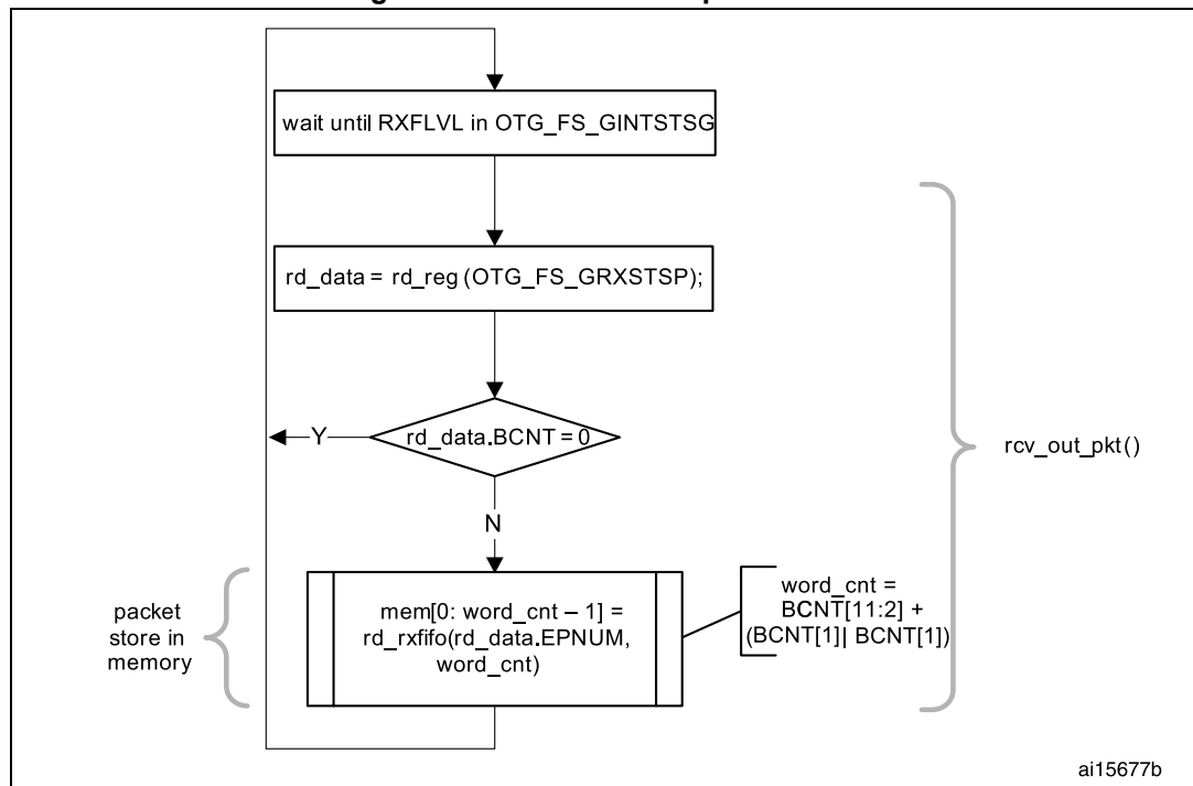
Figure 425. Receive FIFO packet read
