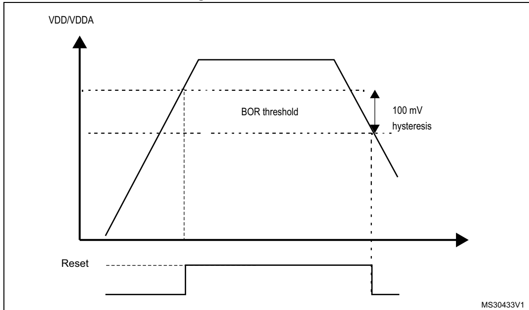
Figure 11. BOR thresholds
