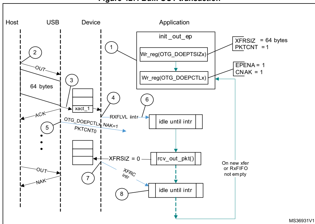
Figure 427. Bulk OUT transaction
