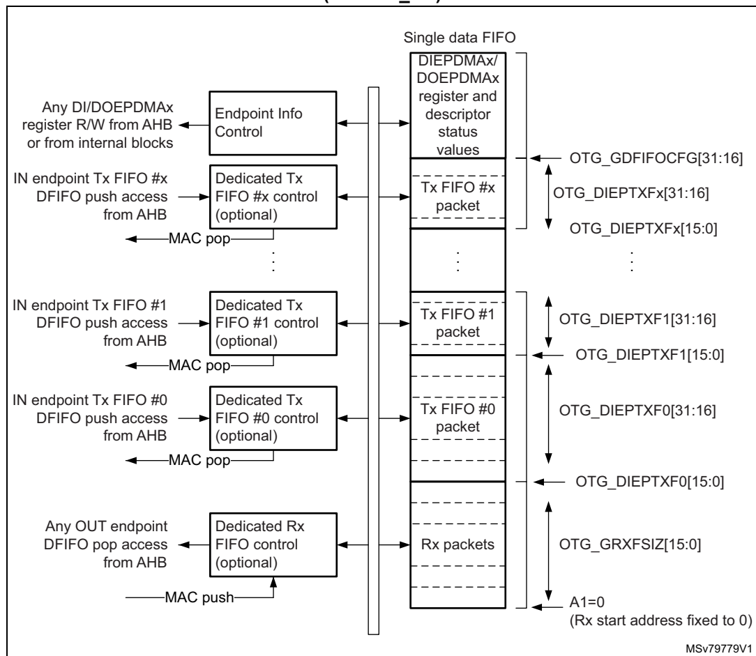
Figure 407. Device-mode FIFO address mapping and AHB FIFO access mapping (for OTG_HS)
