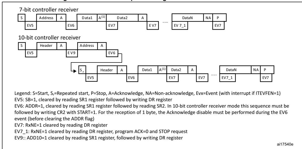
Figure 276. Transfer sequence diagram for controller receiver
