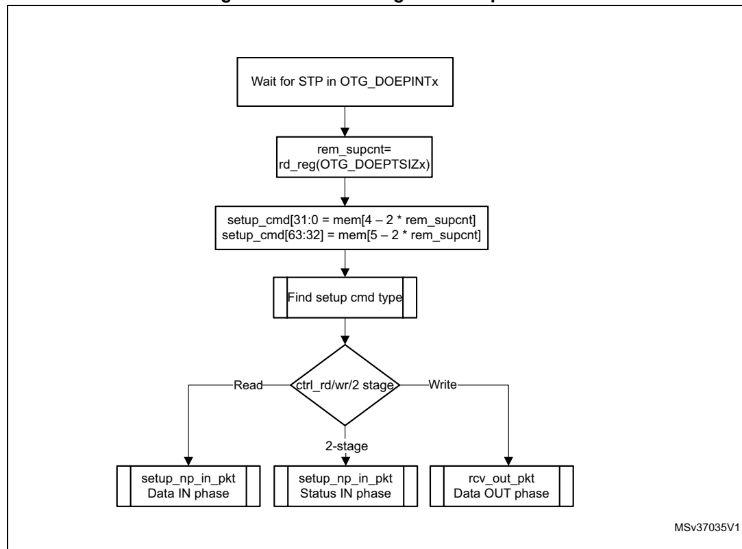
Figure 426. Processing a SETUP packet
