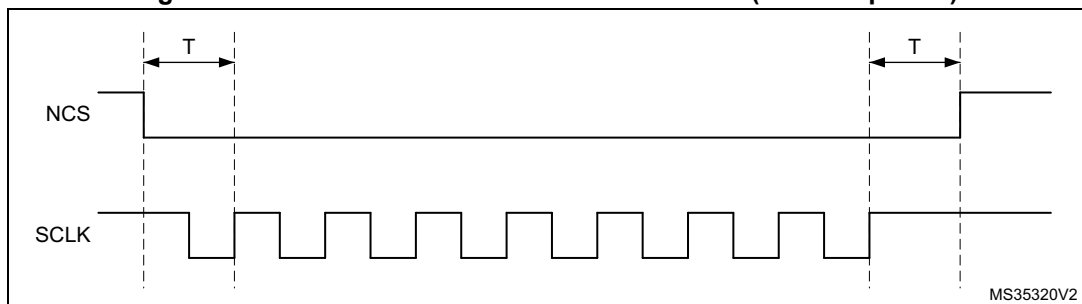
Figure 66. NCS when CKMODE = 1 in SDR mode ( T = \text{CLK period} )
