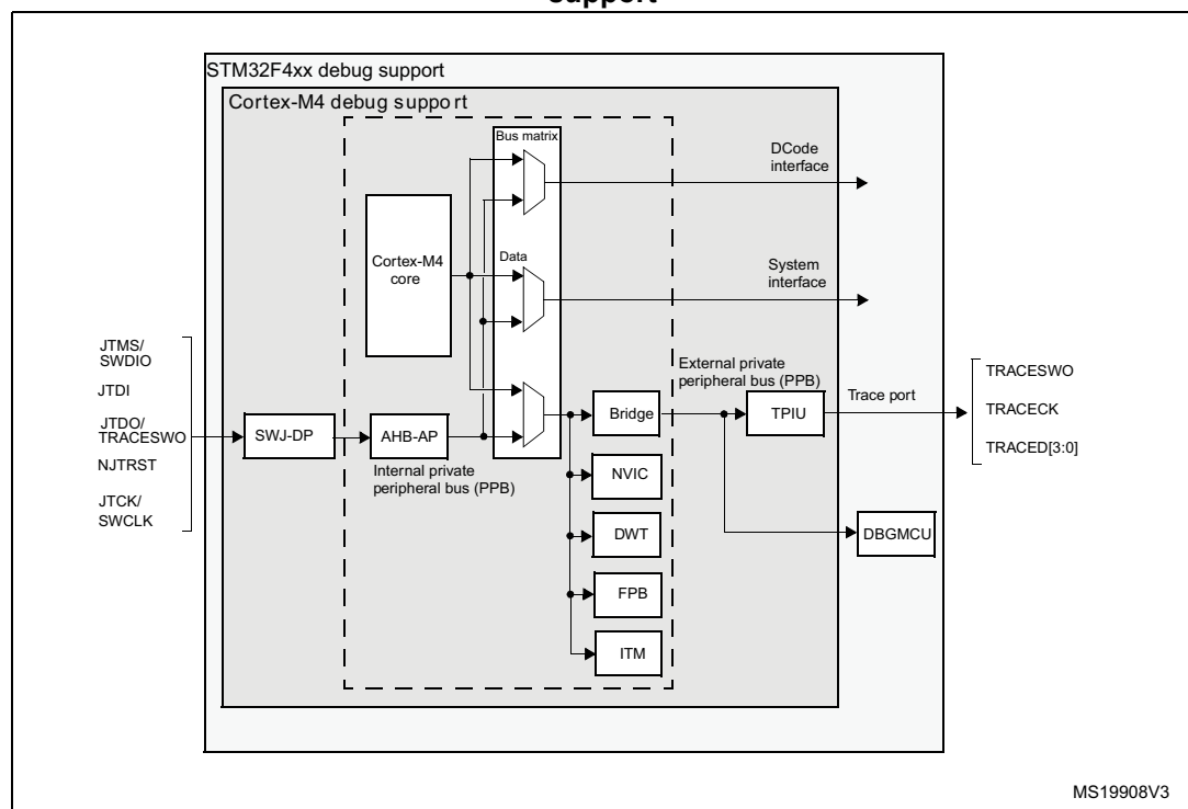
Figure 443. Block diagram of STM32 MCU and Cortex®-M4 with FPU-level debug support
