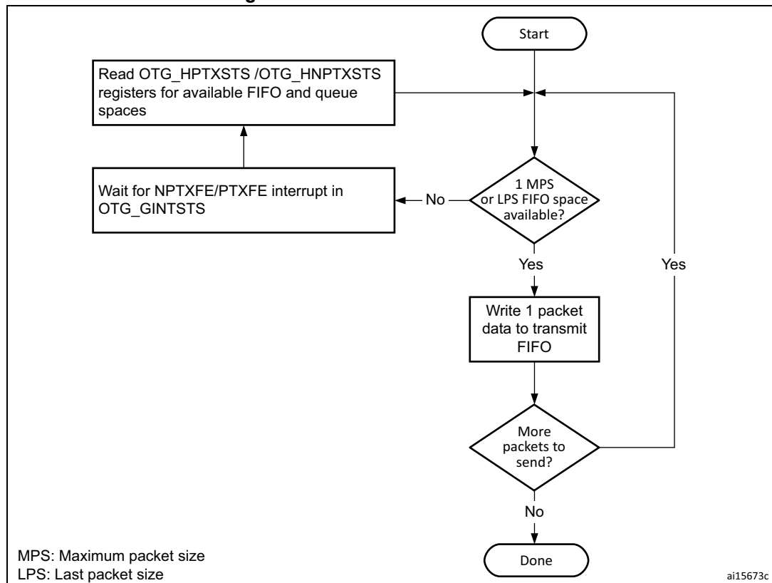
Figure 411. Transmit FIFO write task
