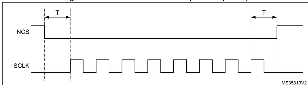
Figure 65. NCS when CKMODE = 0 ( T = \text{CLK period} )
