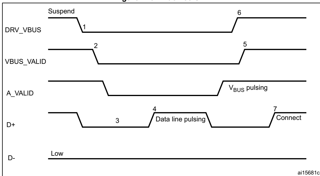
Figure 429. A-device SRP
