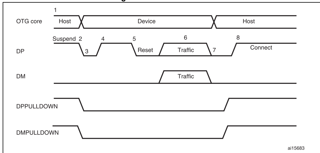
Figure 431. A-device HNP
