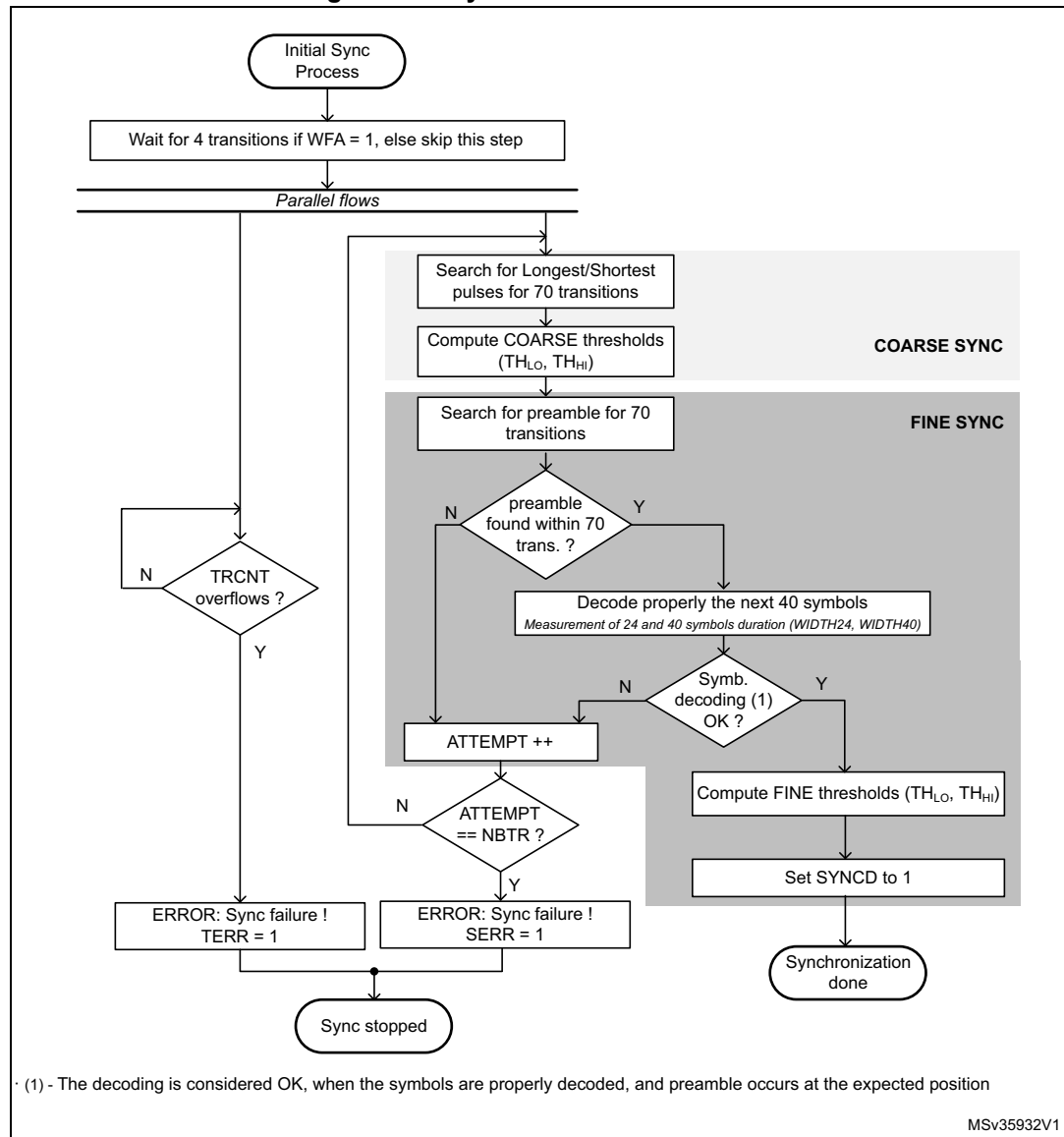
Figure 345. Synchronization flowchart
