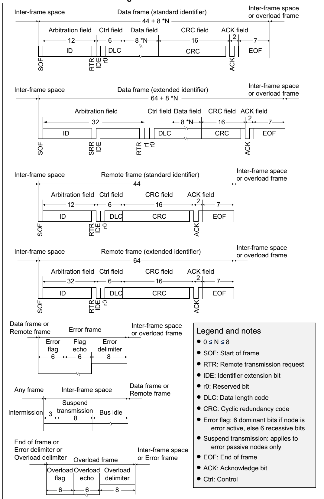
Figure 396. CAN frames
