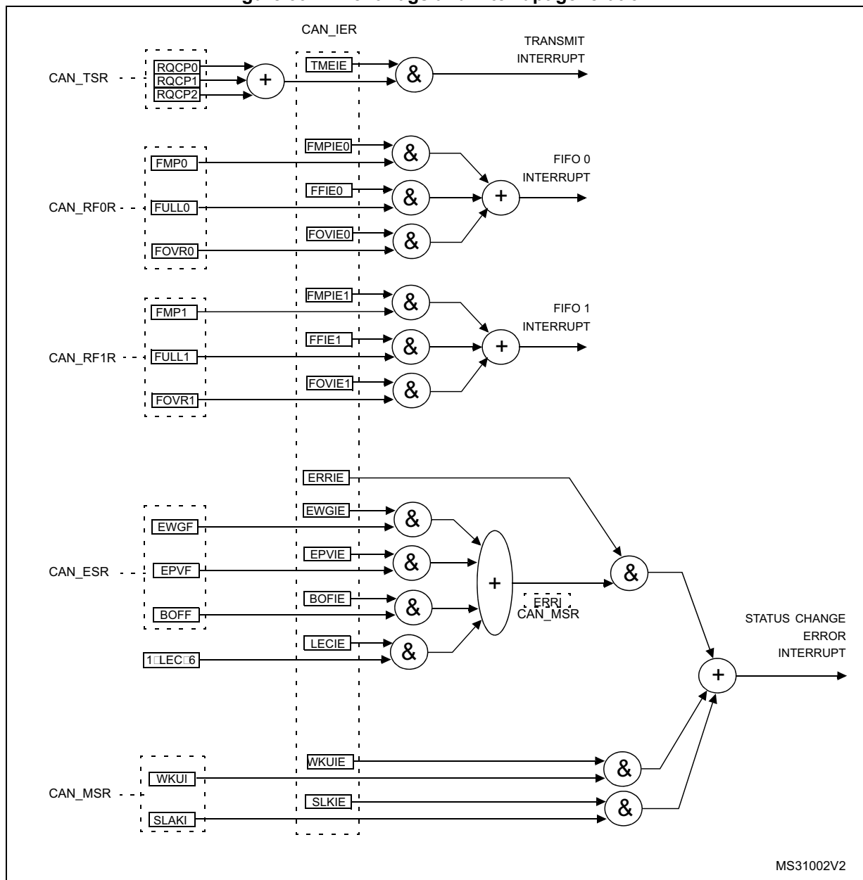
Figure 397. Event flags and interrupt generation
