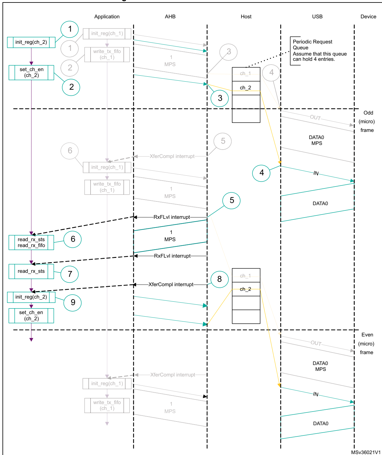
Figure 418. Isochronous IN transactions
