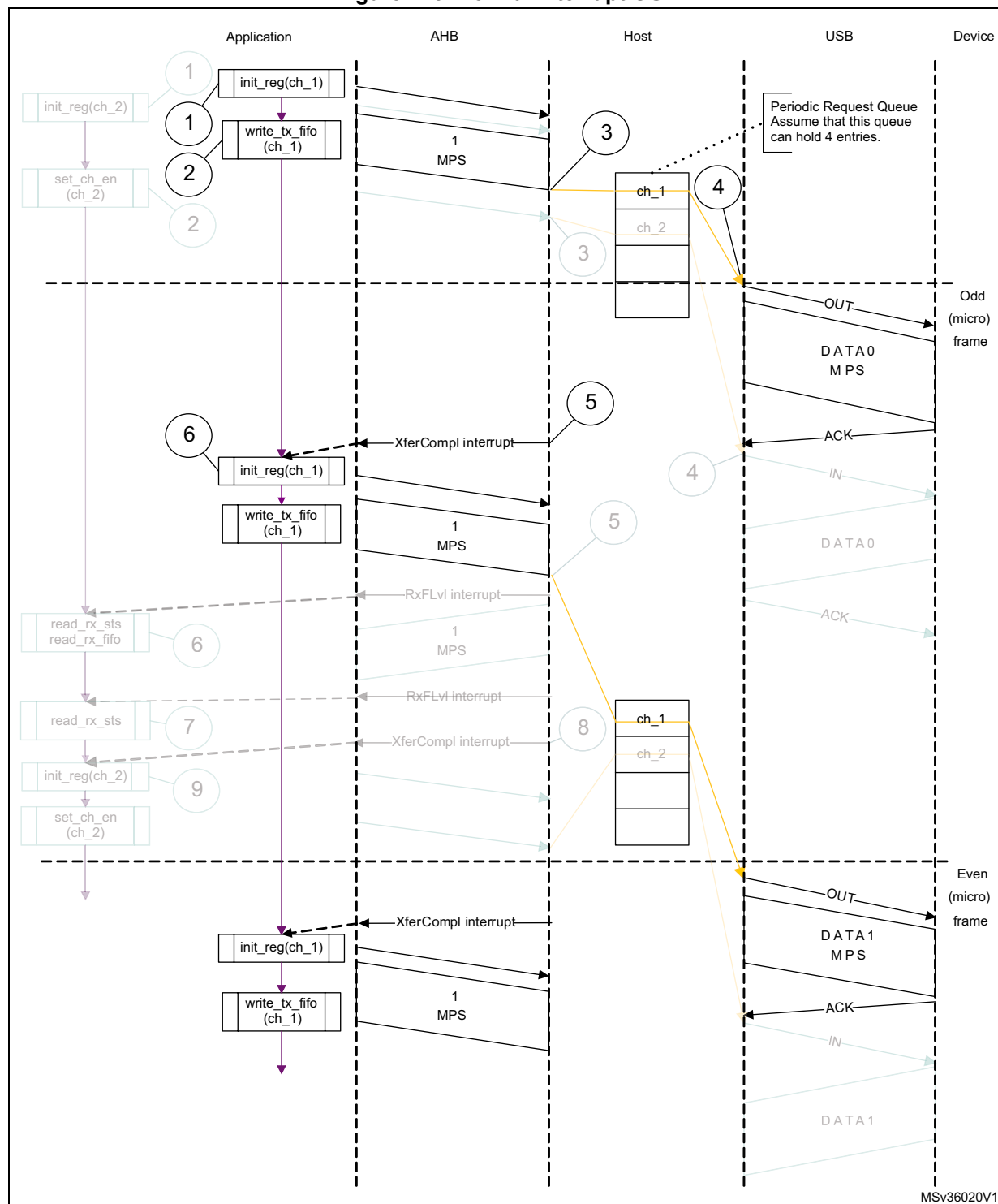
Figure 415. Normal interrupt OUT
