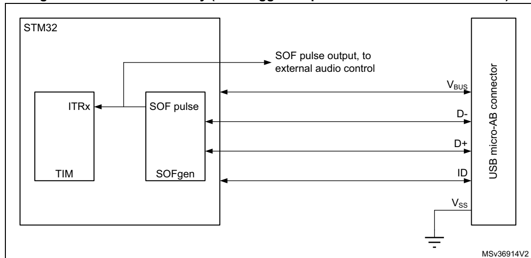
Figure 404. SOF connectivity (SOF trigger output to TIM and ITRx connection)
