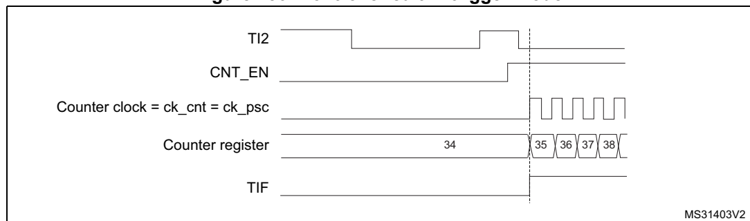
Figure 156. Control circuit in trigger mode
