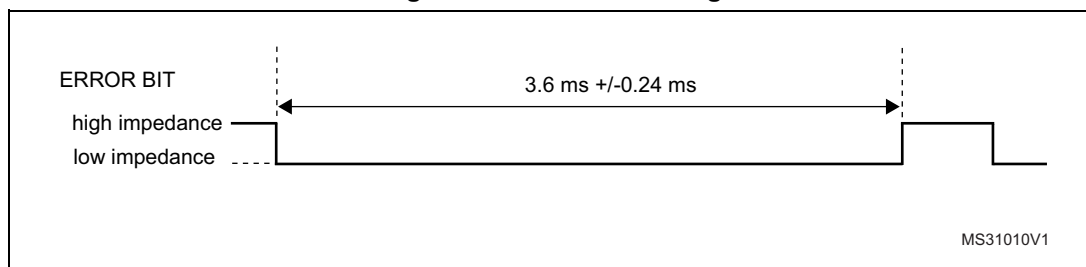
Figure 440. Error bit timing
