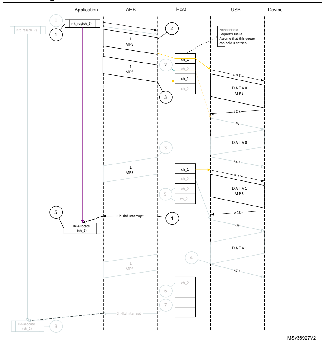
Figure 419. Normal bulk/control OUT/SETUP transactions - DMA
