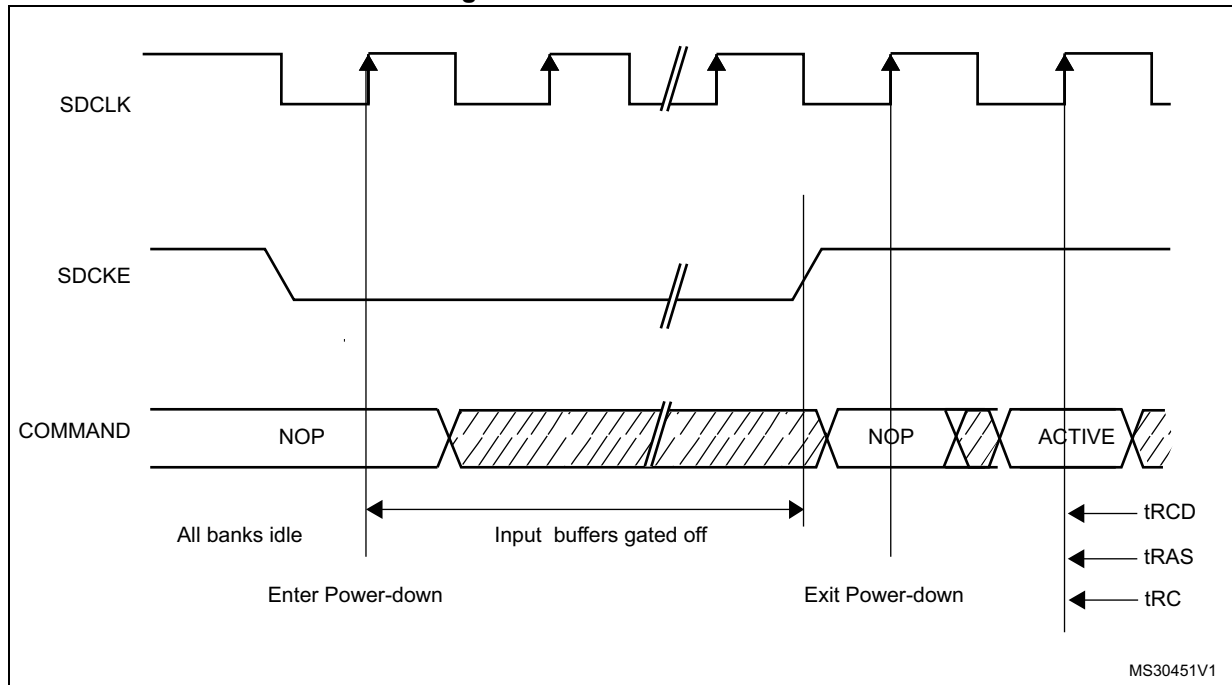
Figure 60. Power-down mode
