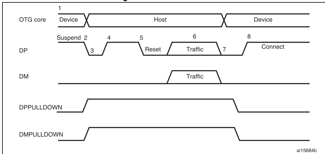
Figure 432. B-device HNP
