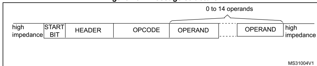
Figure 434. Message structure
