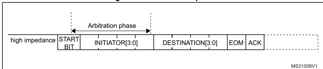
Figure 438. Arbitration phase
