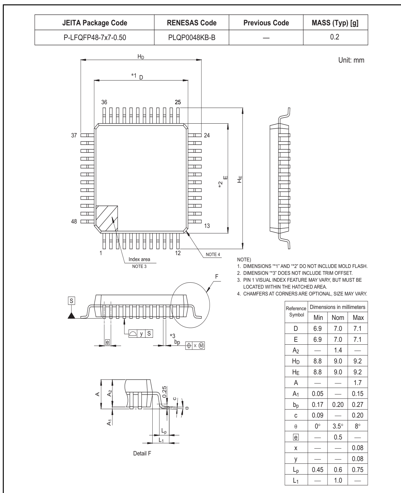
Figure 1.6 48-pin LQFP
