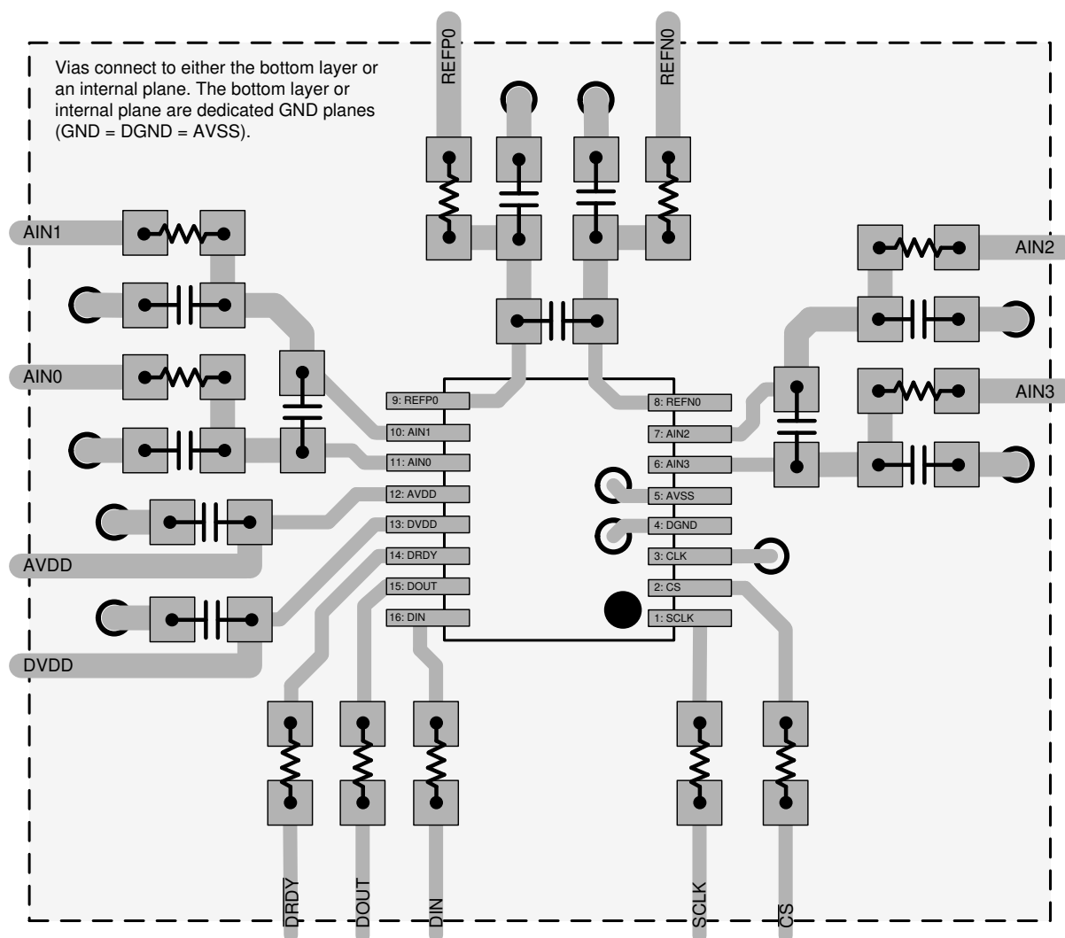
Figure 9-16. Layout Example
