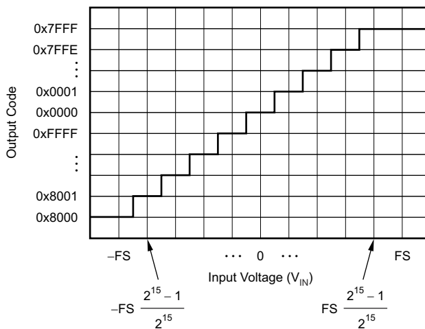
Figure 8-24. Code Transition Diagram
