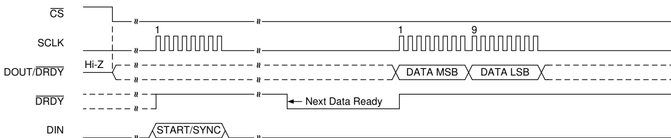
Figure 8-27. Single-Shot Conversion Mode ( \text{DRDYM} = 0\text{b} )
