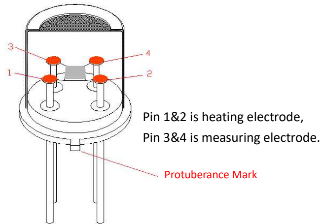
Fig8.Pin Schematic Diagram
