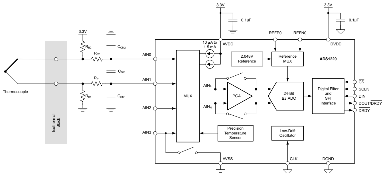
Figure 9-3. Thermocouple Measurement
