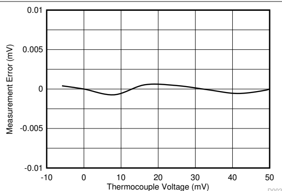
Figure 9-4. Voltage Measurement Error vs V_{TC}
