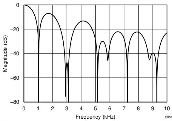
Figure 8-21. Filter Response (DR = 1kSPS)
