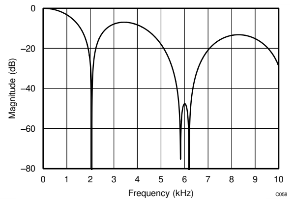
Figure 8-22. Filter Response (DR = 2kSPS)
