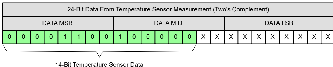
Figure 8-23. 14-Bit Temperature Sensor Data Alignment Within 24-Bit Conversion Result
