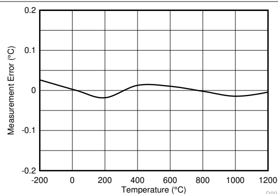
Figure 9-5. Temperature Measurement Error vs T_{TC}
