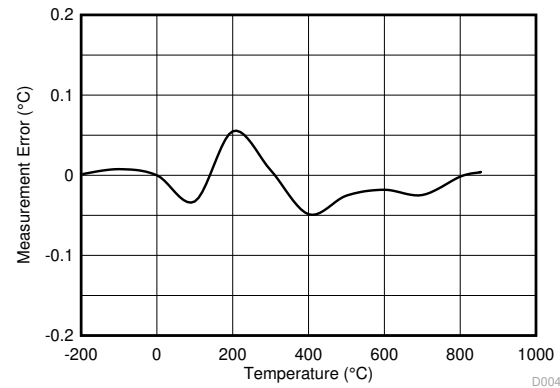
Figure 9-10. Temperature Measurement Error vs T_{\text{RTD}}
