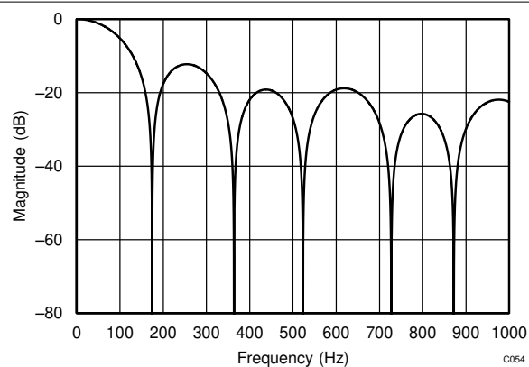
Figure 8-18. Filter Response (DR = 175SPS)
