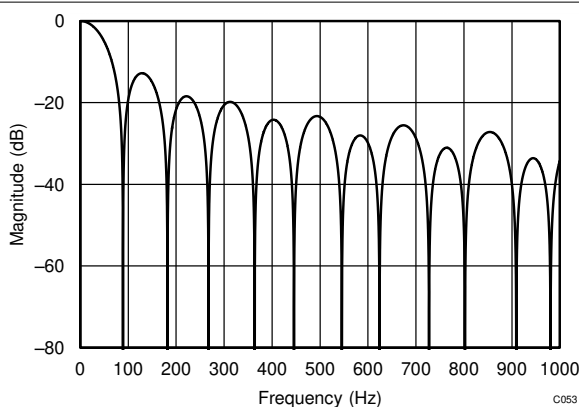
Figure 8-17. Filter Response (DR = 90SPS)
