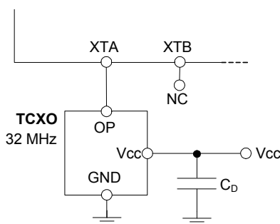
Figure 39. TCXO Connection
