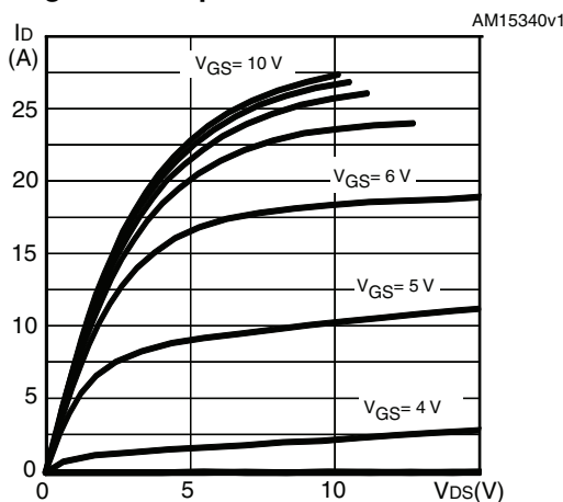
Figure 6. Output characteristics
