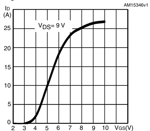
Figure 7. Transfer characteristics
