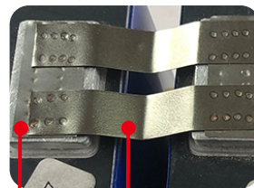
4. Check the spots' reliability. Finish spot welding.
