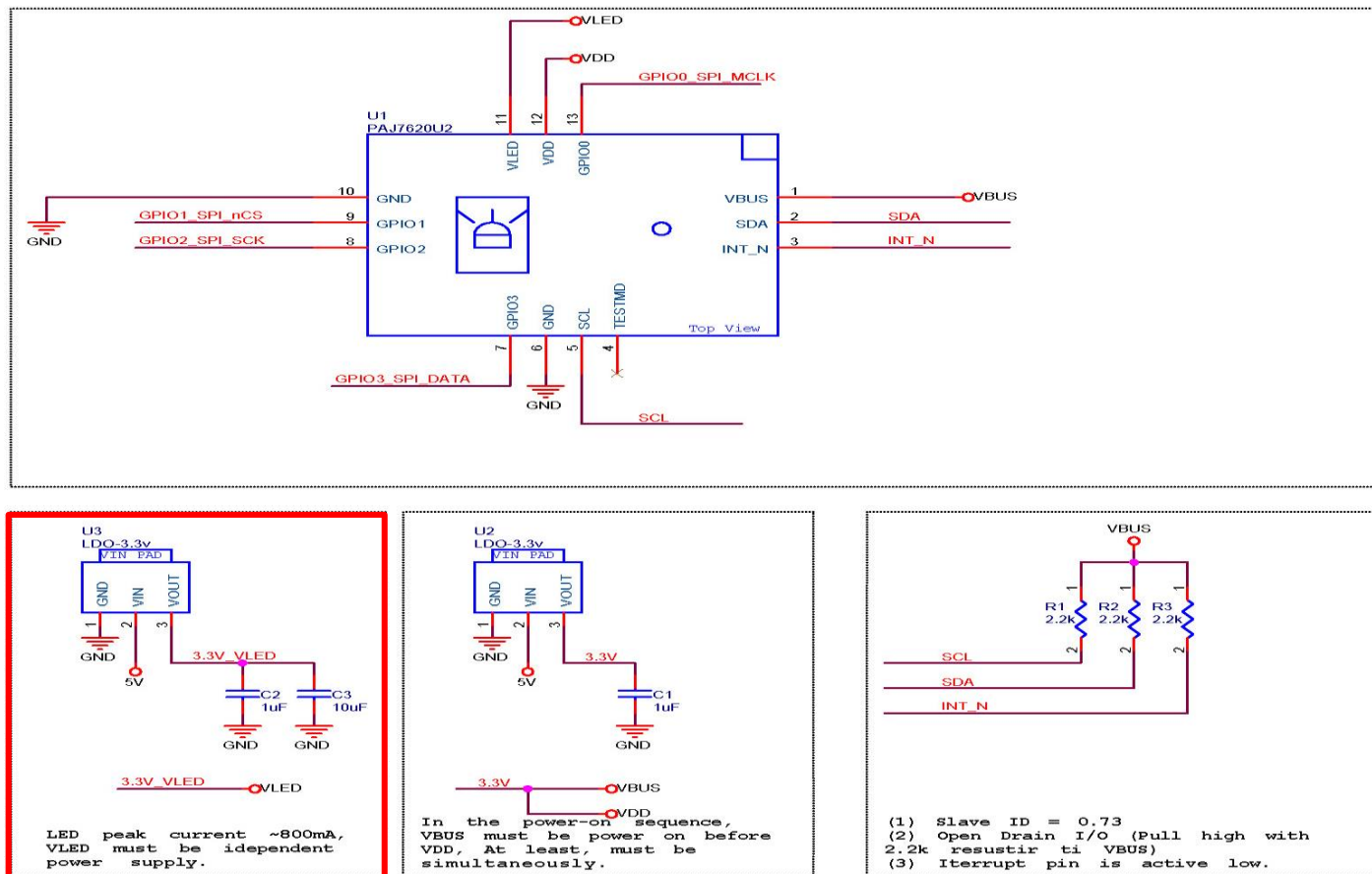
Figure 7. PAJ7620U2 Application Circuit
