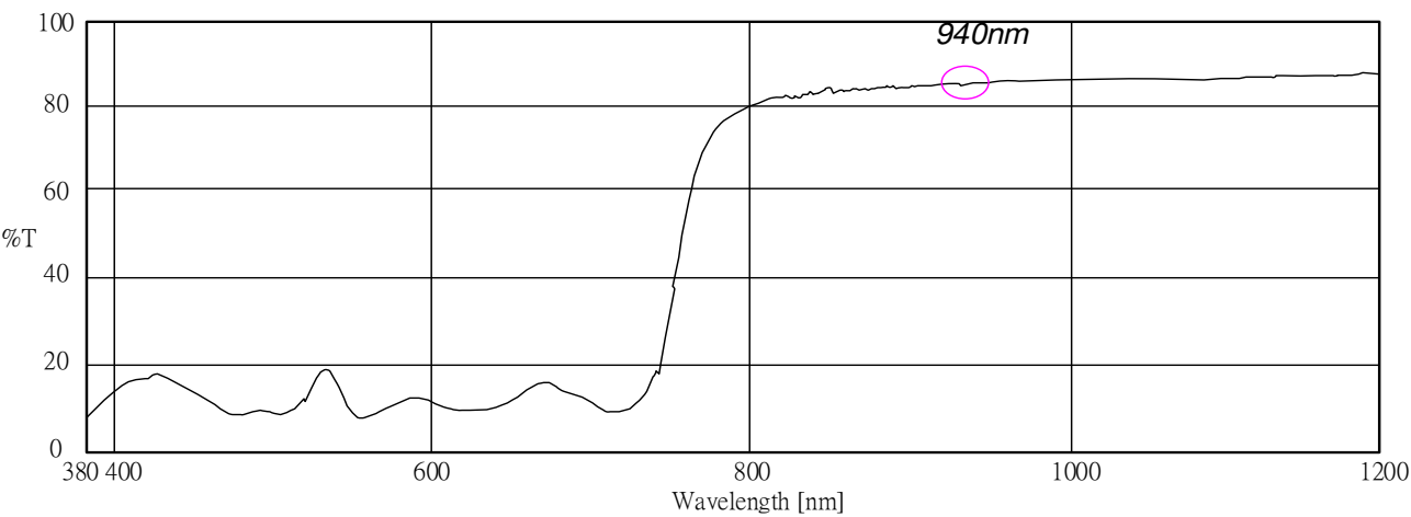
Figure 6. IR Ink Spectrum
