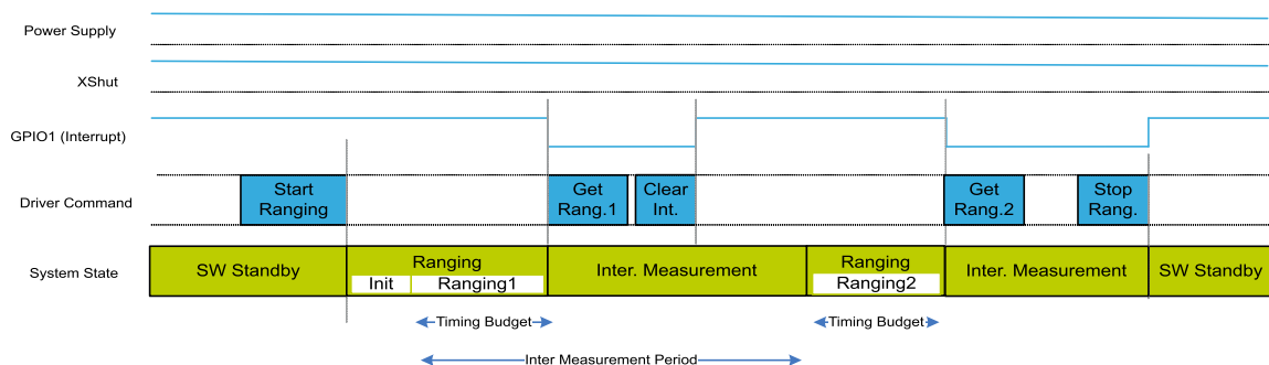
Figure 9. Autonomous sequence
