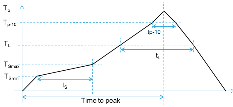
Figure 23. Solder profile
