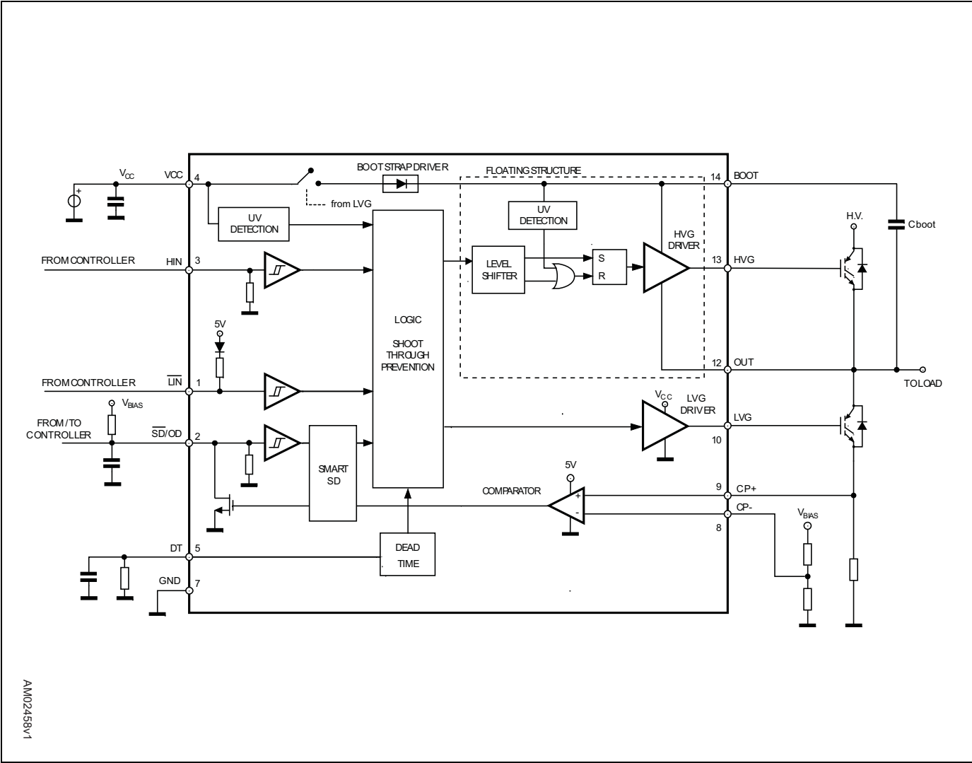
Figure 9. Application diagram
