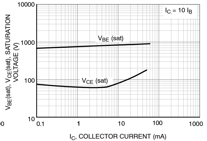
Figure 2. Base-Emitter Saturation Voltage and Collector-Emitter Saturation Voltage
