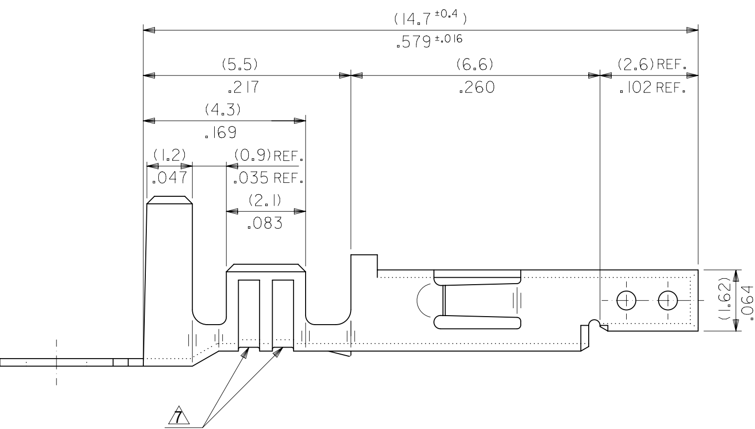
#18-24 TERMINAL SHOWN
