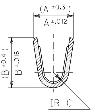
SECT. G-G
