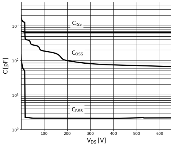
Figure 6. Typical Capacitance
