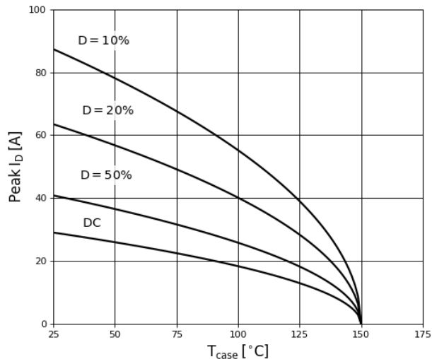
Figure 11. Current Derating
