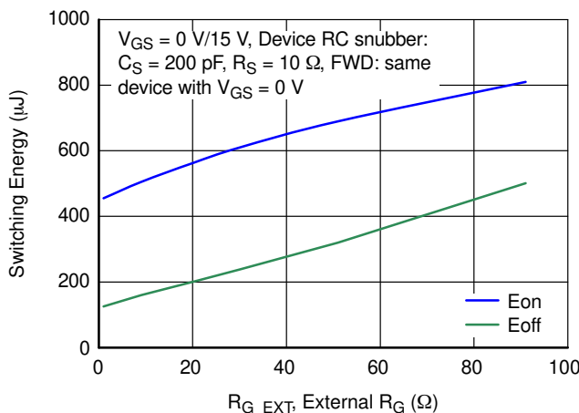
Figure 23. Clamped Inductive Switching Energies vs. R_{G,EXT} at V_{DS} = 400\text{ V} , I_D = 40\text{ A} and T_J = 25\text{ °C}
