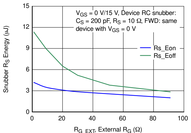
Figure 24. RC Snubber Energy Losses vs. R_{G,EXT} at V_{DS} = 400\text{ V} , I_D = 40\text{ A} and T_J = 25\text{ °C}
