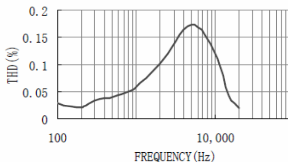
THD vs Frequency T=25°C, Vdd=3.3V, RL=4 Ω, and Po=425mW
