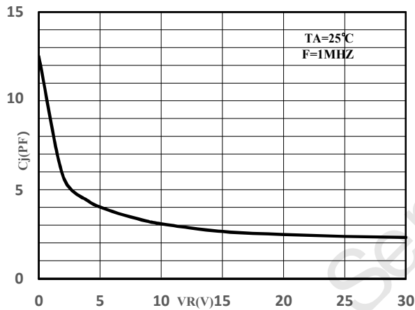
Fig.3-Capacitance Characteristics
