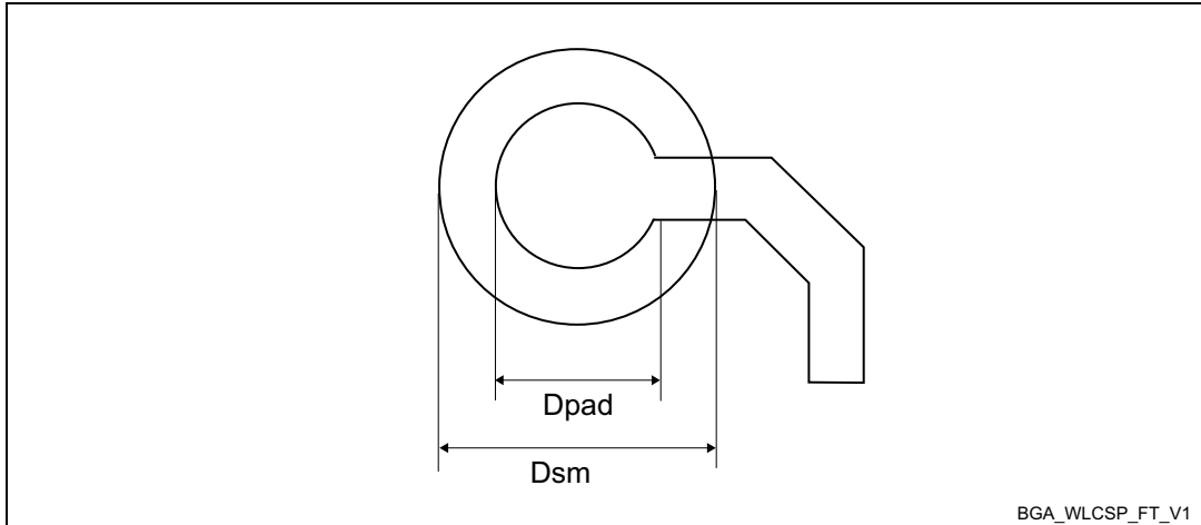
Figure 58. UFBGA100 - Footprint example
