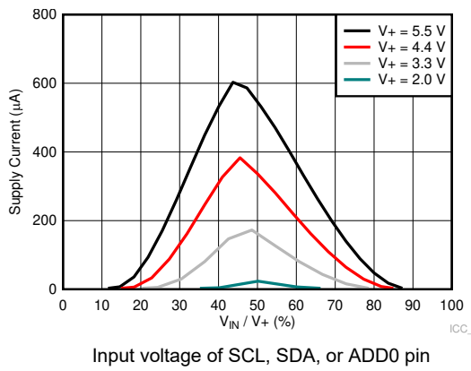
Figure 6-12. Supply Current vs Input Cell Voltage
