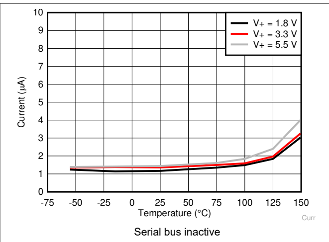
Figure 6-7. Quiescent Current in Standby Mode
