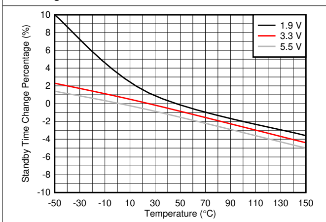
Figure 6-10. Standby Time vs Temperature
