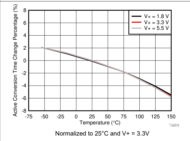
Figure 6-9. Active Conversion Time vs Temperature
