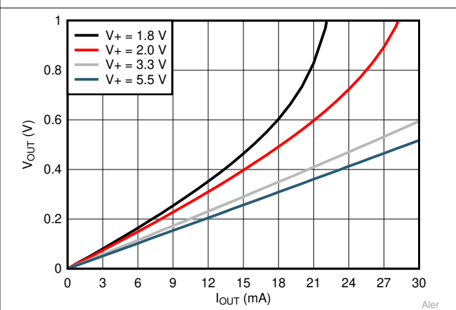
Figure 6-11. ALERT Pin Output Voltage vs Pin Sink Current
