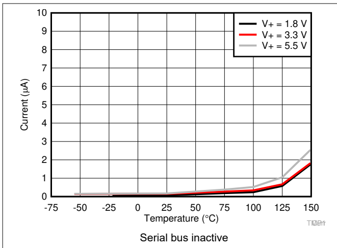
Figure 6-6. Quiescent Current in Shutdown Mode
