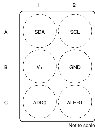
Figure 5-1. YBG Package 6-Pin DSBGA Top View
