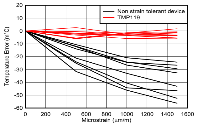
Figure 6-13. Temperature Error vs Microstrain
