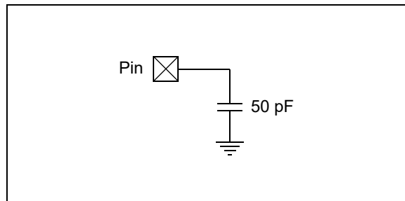
FIGURE 4-2: LOAD CONDITIONS FOR DEVICE TIMING SPECIFICATIONS
