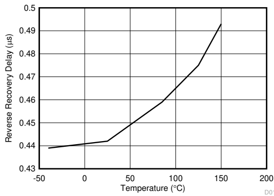
Figure 7-9. Reverse Current Blocking Delay vs Temperature
