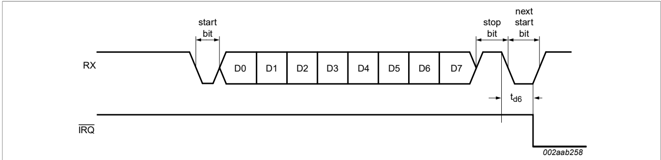
Figure 26. Receive interrupt
