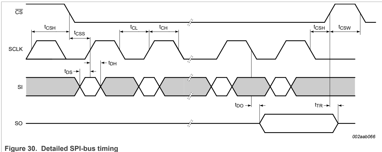
Figure 30. Detailed SPI-bus timing
