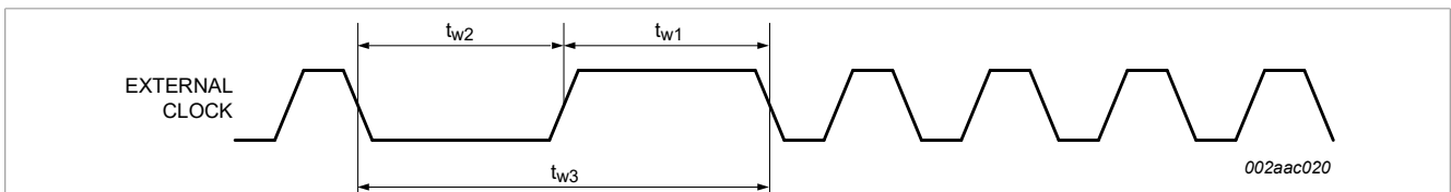
Figure 29. External clock timing
