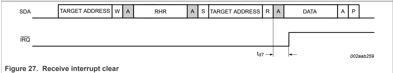
Figure 27. Receive interrupt clear
