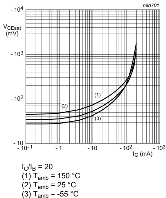
Fig. 5. PNP TR2: Collector-emitter saturation voltage as a function of collector current; typical values
