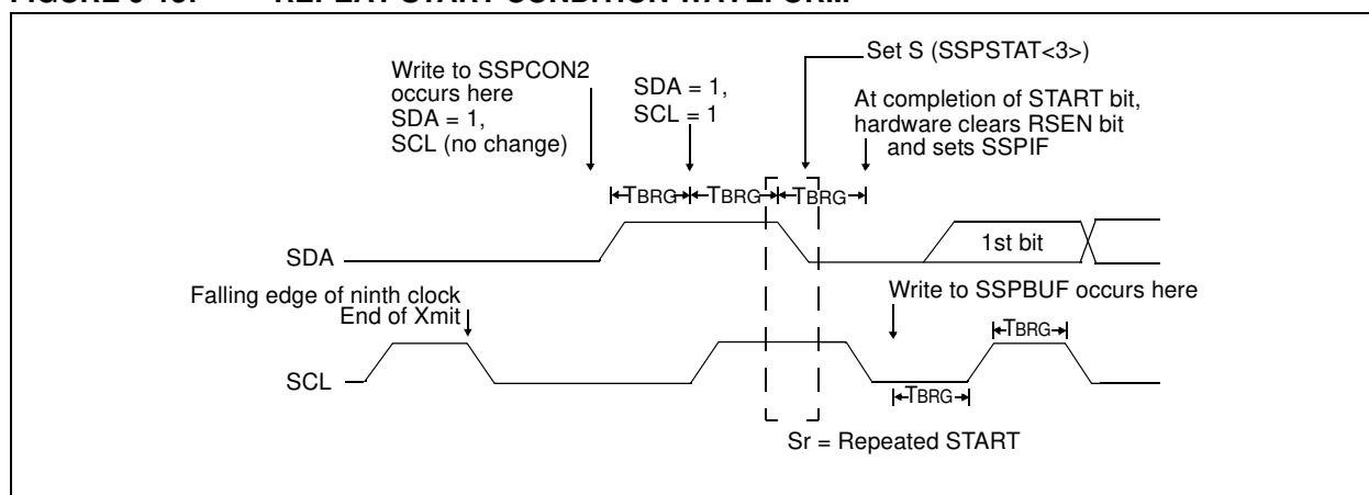
FIGURE 9-13: REPEAT START CONDITION WAVEFORM
