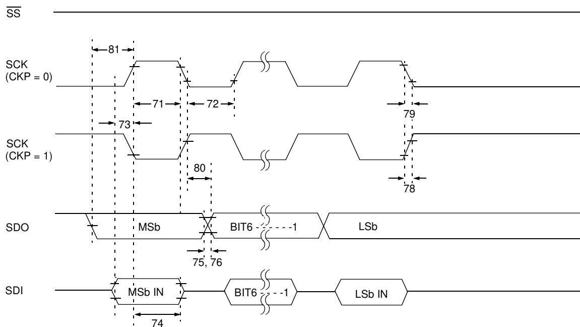
FIGURE 15-14: SPI MASTER MODE TIMING (CKE = 1, SMP = 1)
