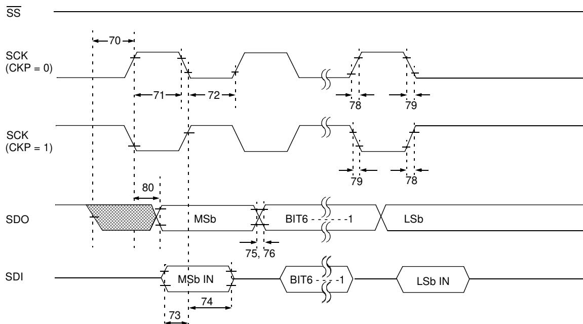
FIGURE 15-13: SPI MASTER MODE TIMING (CKE = 0, SMP = 0)
