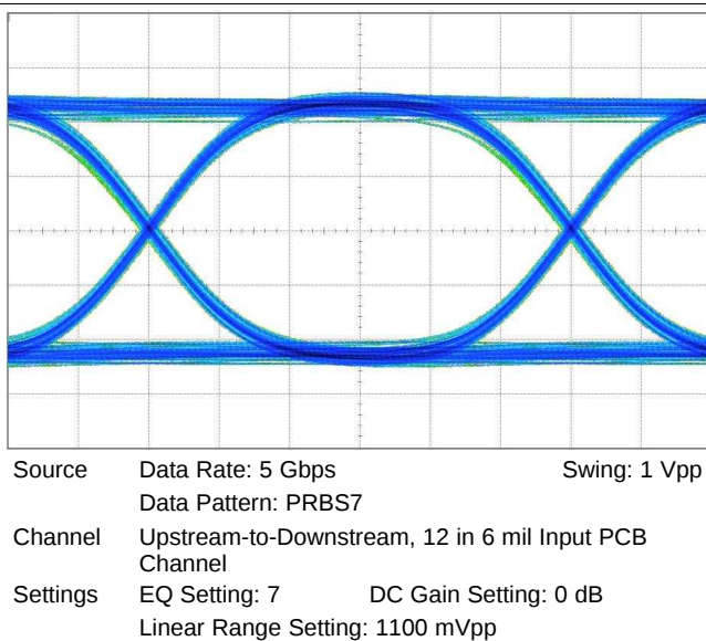
Figure 17. Output Eye-Pattern Performance at 5 Gbps
