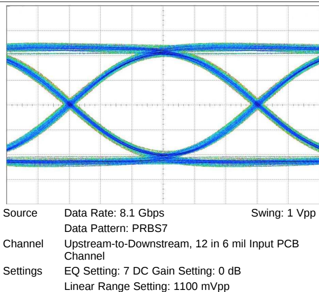
Figure 18. Output Eye-Pattern Performance at 8.1 Gbps
