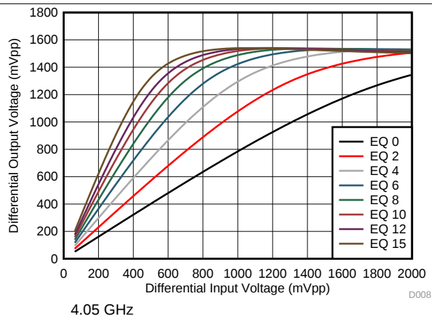
Figure 12. Downstream-to-Upstream Linearity Performance at 4.05 GHz
