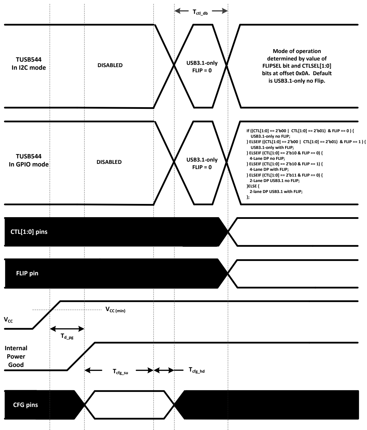
Figure 21. Power-Up Timing
