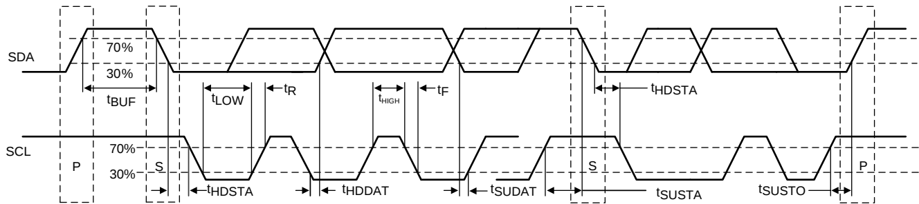
Figure 1. I²C Timing Diagram Definitions
