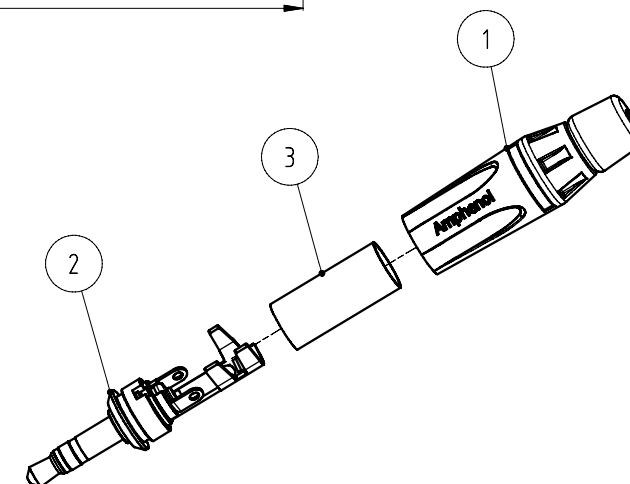
EXPLORED VIEW ( 1 : 1 )
