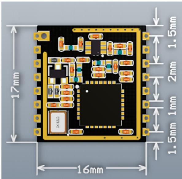
Figure 4 Plan view of Ra-01 module size
