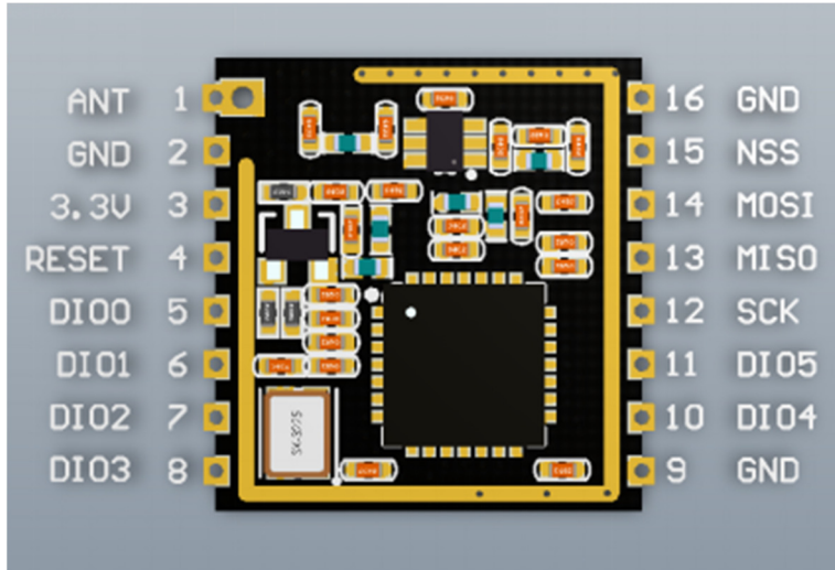
Figure 2 Ra-01 pin diagram
