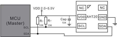
Figure 16 Typical application circuit
