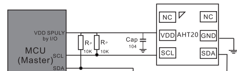
Figure 15-1 Typical application circuit ①, the pull-up voltage and VDD of SCL and SDA are powered by the MCU.
