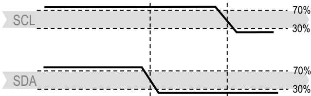
Figure 18 Start Transmit State (S) - When SCL is at high level, SDA is converted from high level to low level. The start state is a special bus state controlled by the main engine, indicating the start of slave machine transit (after Start, BUS is generally considered to be in a busy state).
