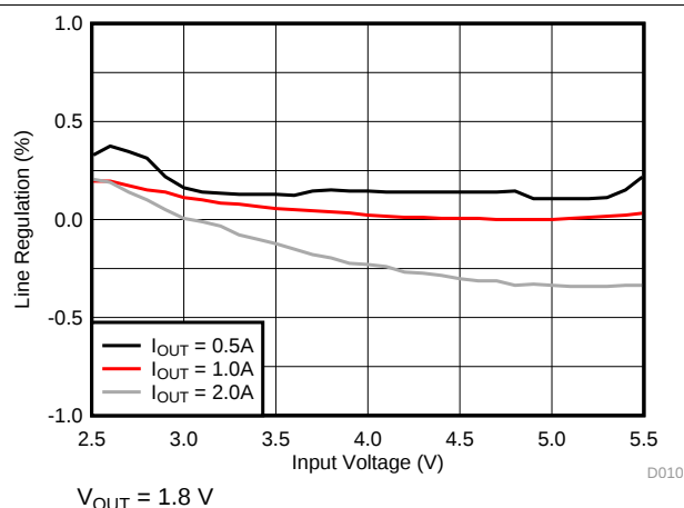
Figure 11. Line Regulation
