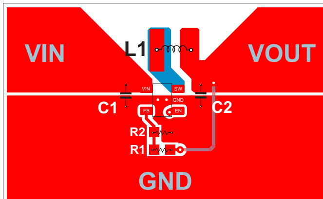
Figure 20. TLV62569DBV Layout
