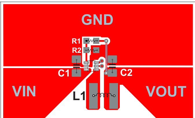
Figure 21. TLV62569PDRL Layout
