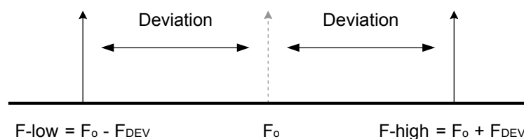
Figure 12. (G)FSK Deviation
