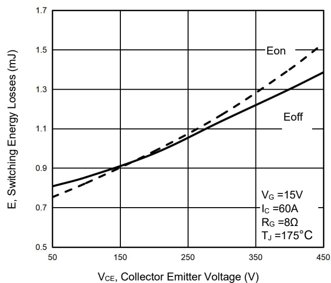
Figure 20 Switching Loss vs. V_{CE}
