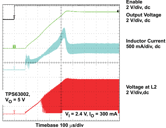
Figure 19. Start-Up After Enable (TPS63002)
