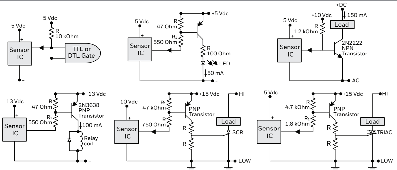
Figure 5. Wiring Diagrams
