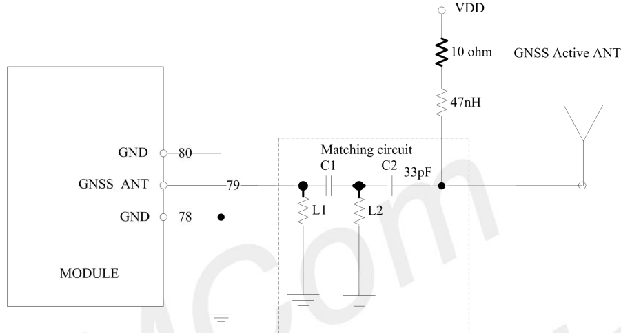
Figure 37: Active antenna circuit
