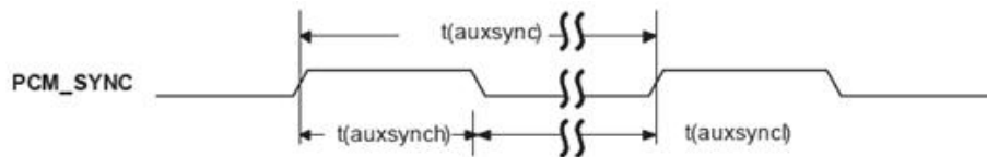
Figure 25: PCM_SYNC timing
