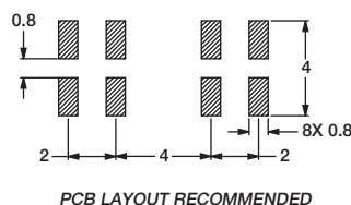
PCB LAYOUT RECOMMENDED
