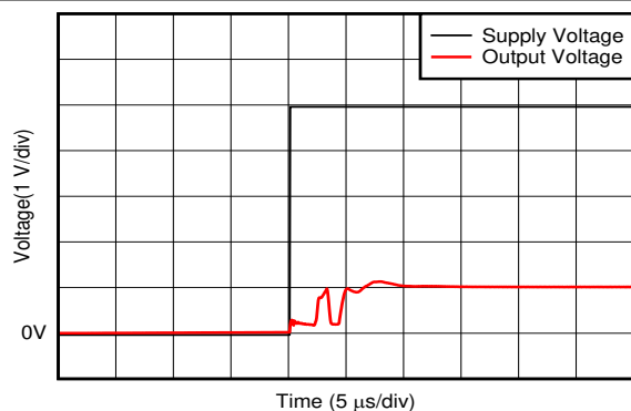
Figure 6-33. Start-Up Response
