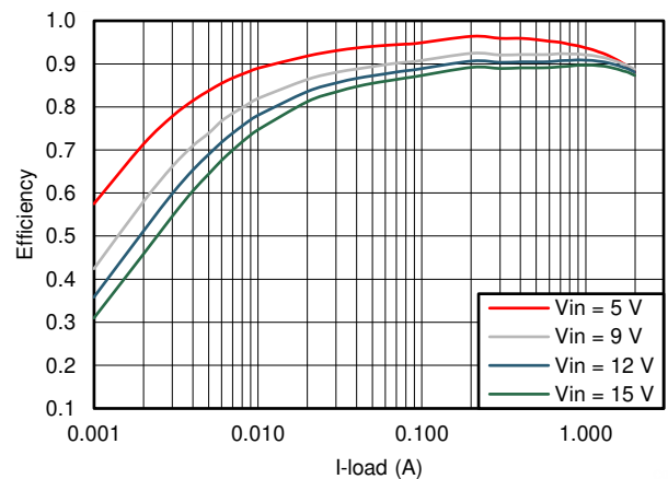
Figure 5-12. TPS562201 V_{OUT} = 3.3 V Efficiency, L = 2.2 \mu\text{H}
