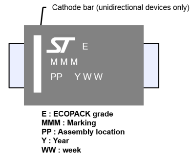
Figure 15. SMA marking
