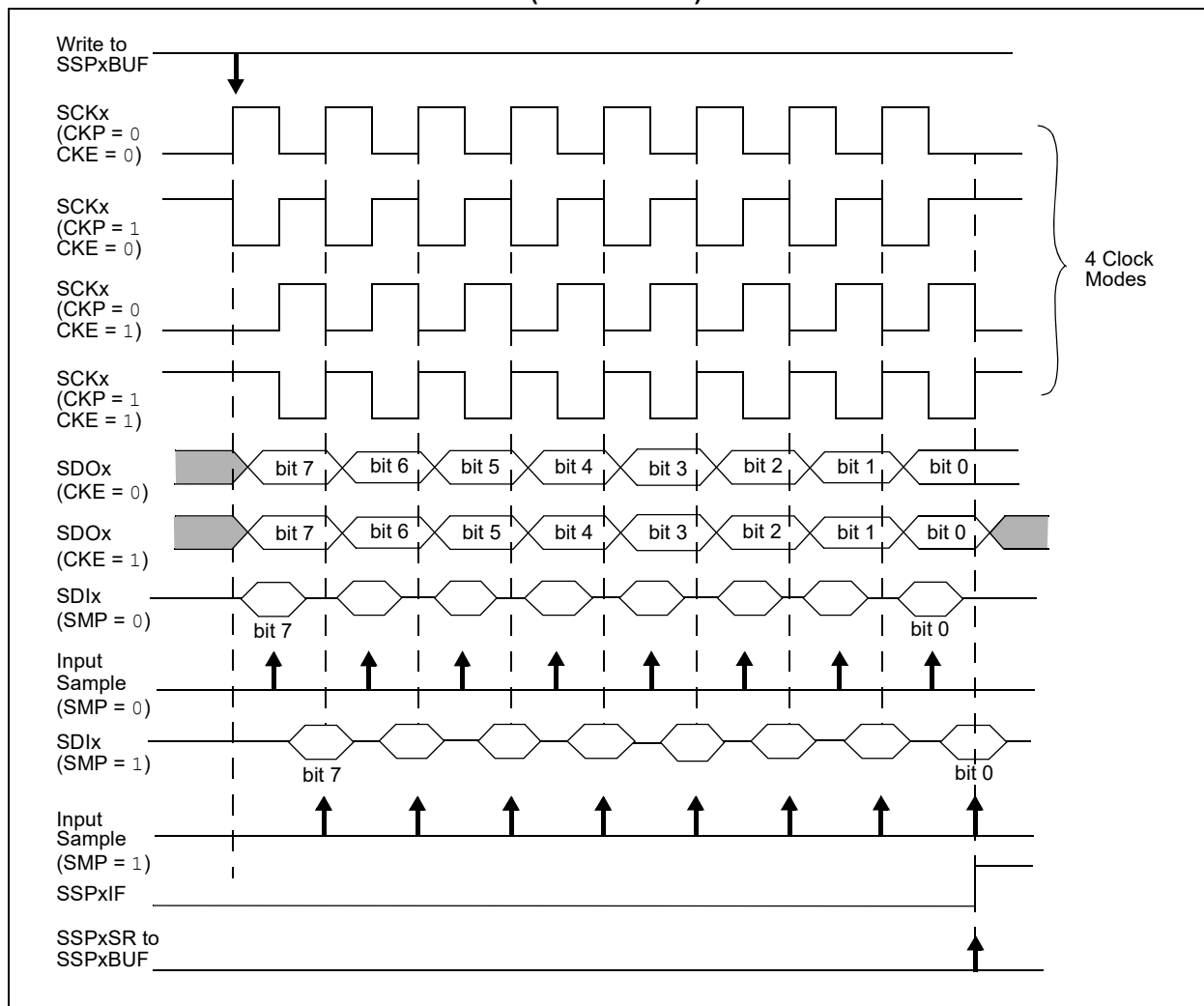
FIGURE 15-6: SPI MODE WAVEFORM (HOST MODE)
