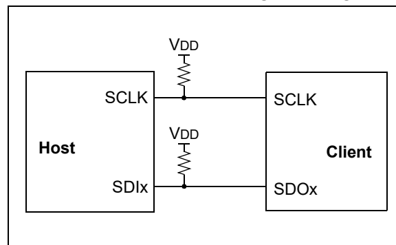
FIGURE 15-11: I 2 C HOST/CLIENT CONNECTION
