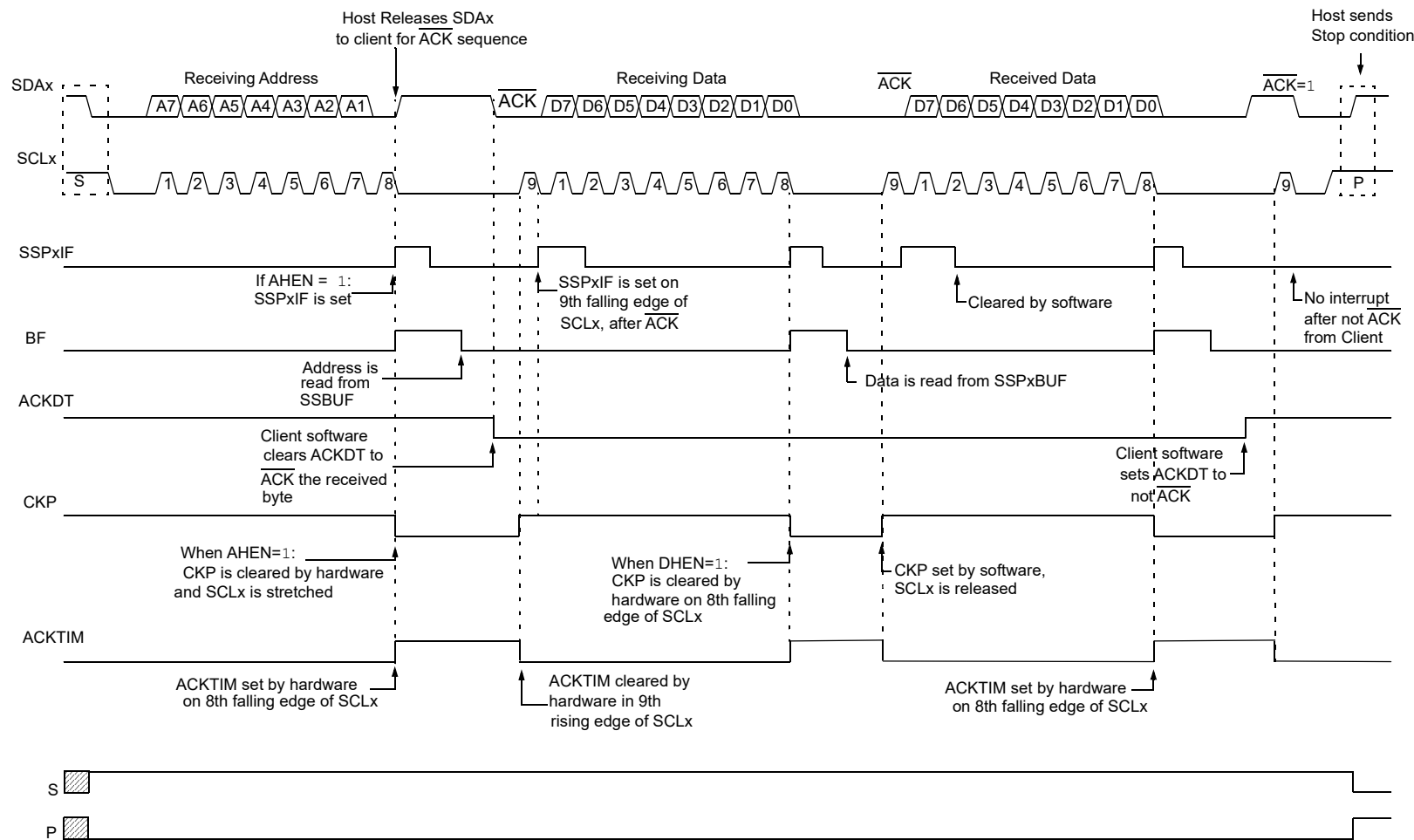
FIGURE 15-16: I 2 C CLIENT, 7-BIT ADDRESS, RECEPTION (SEN = 0, AHEN = 1, DHEN = 1)
