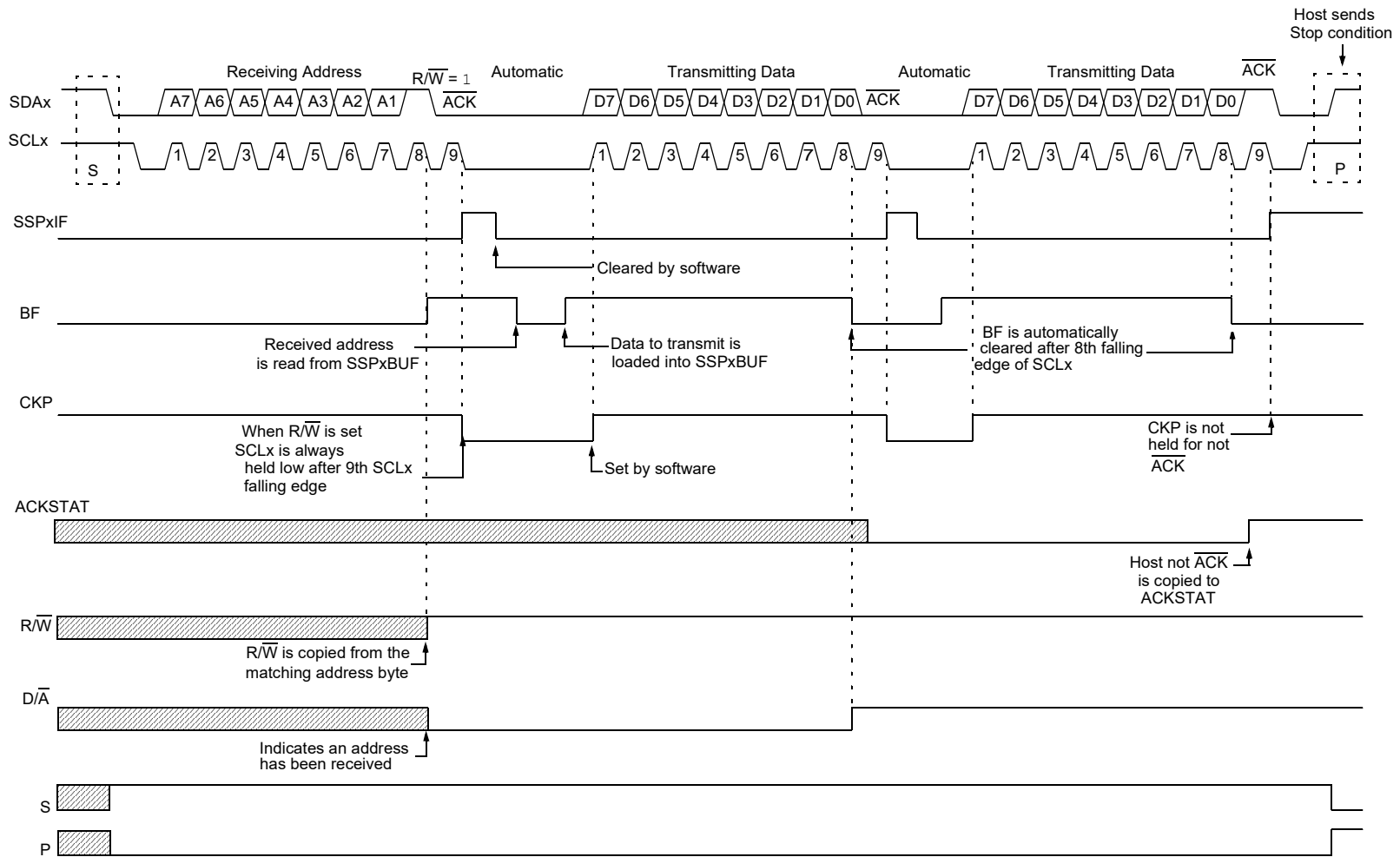
FIGURE 15-18: I 2 C CLIENT, 7-BIT ADDRESS, TRANSMISSION (AHEN = 0)
