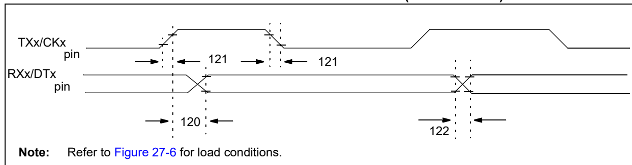
FIGURE 27-21: EUSART SYNCHRONOUS TRANSMISSION (HOST/CLIENT) TIMING
