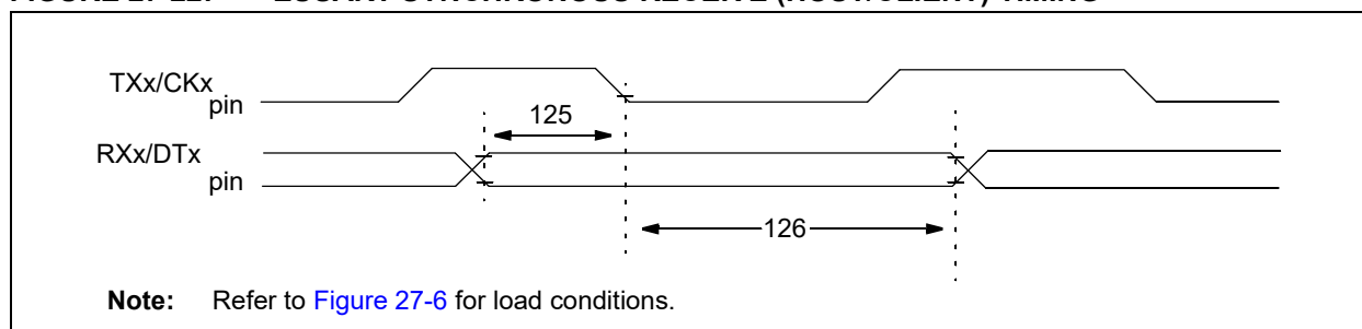
FIGURE 27-22: EUSART SYNCHRONOUS RECEIVE (HOST/CLIENT) TIMING
